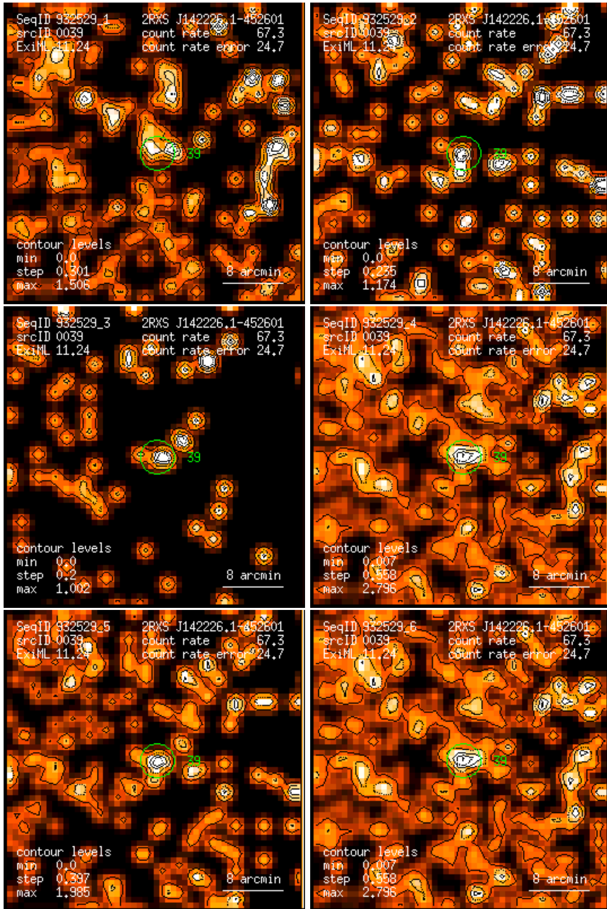
Figure 39: RASS 932529: detection 0039: band rate images, Gaussian filter: (1) PSPC channels 11 – 41, (2) 52 – 90, (3) 91 – 201, (4) 11 – 235, (5) 52 – 201, (6) 11 – 201. Broad band rates in counts/ks. Band rate contour levels in counts/ks/arcmin 2 .
