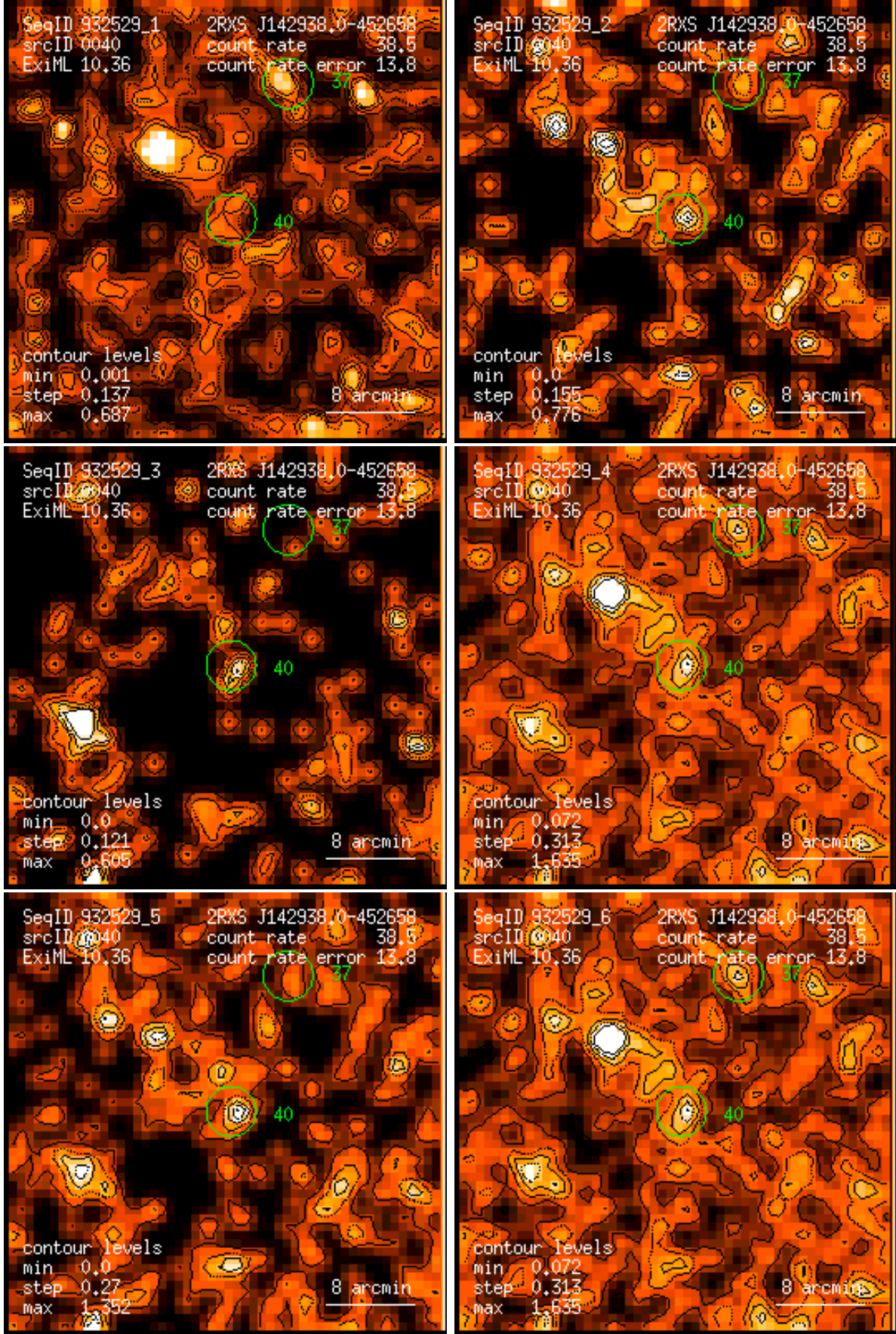
Figure 40: RASS 932529: detection 0040: band rate images, Gaussian filter: (1) PSPC channels 11 – 41, (2) 52 – 90, (3) 91 – 201, (4) 11 – 235, (5) 52 – 201, (6) 11 – 201. Broad band rates in counts/ks. Band rate contour levels in counts/ks/arcmin 2 .
