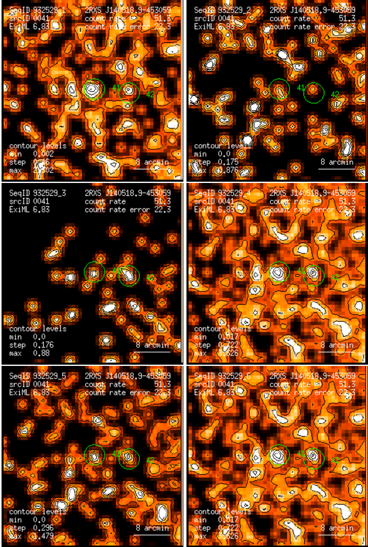
Figure 41: RASS 932529: detection 0041: band rate images, Gaussian filter: (1) PSPC channels 11 – 41, (2) 52 – 90, (3) 91 – 201, (4) 11 – 235, (5) 52 – 201, (6) 11 – 201. Broad band rates in counts/ks. Band rate contour levels in counts/ks/arcmin 2 .
