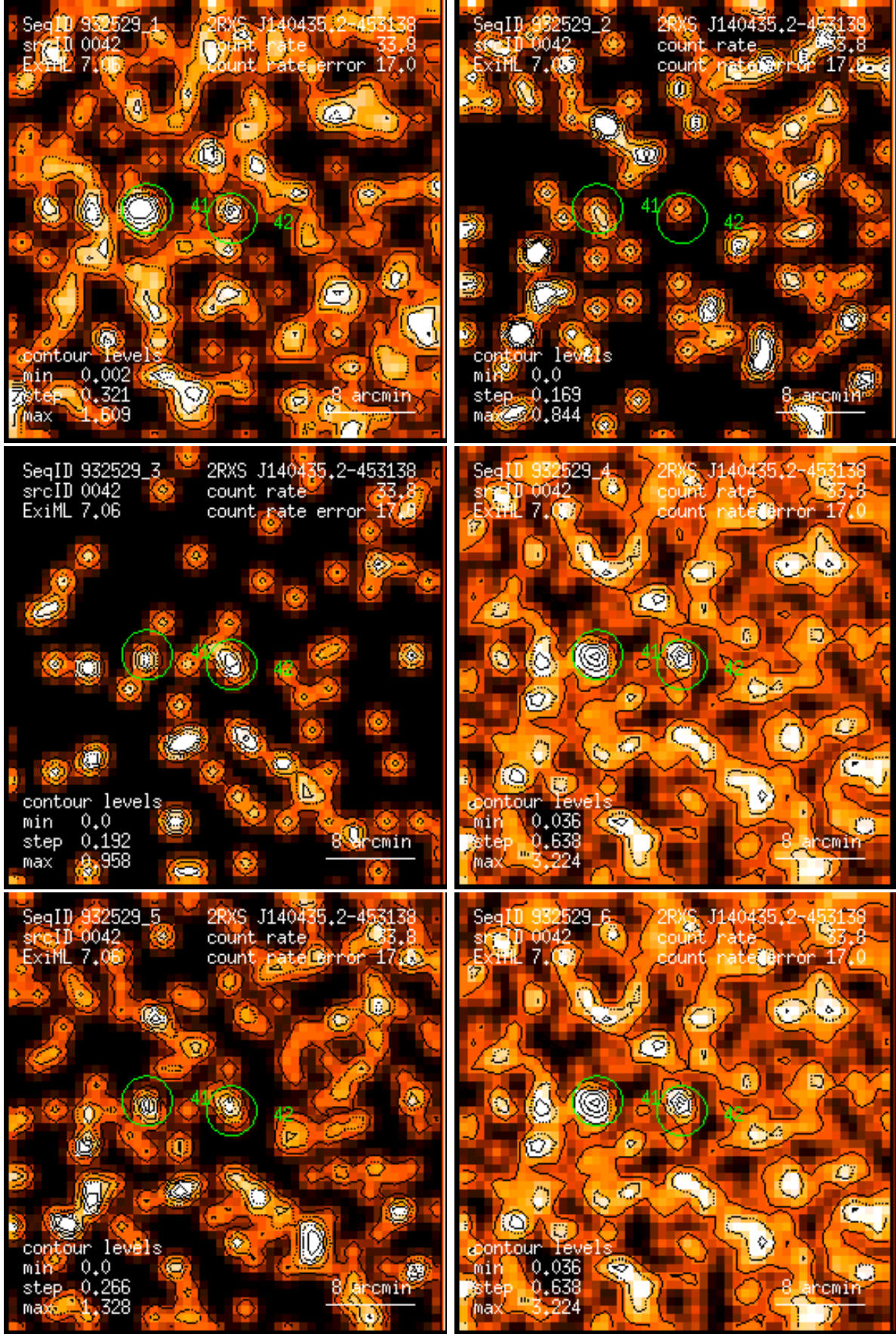
Figure 42: RASS 932529: detection 0042: band rate images, Gaussian filter: (1) PSPC channels 11 – 41, (2) 52 – 90, (3) 91 – 201, (4) 11 – 235, (5) 52 – 201, (6) 11 – 201. Broad band rates in counts/ks. Band rate contour levels in counts/ks/arcmin 2 .
