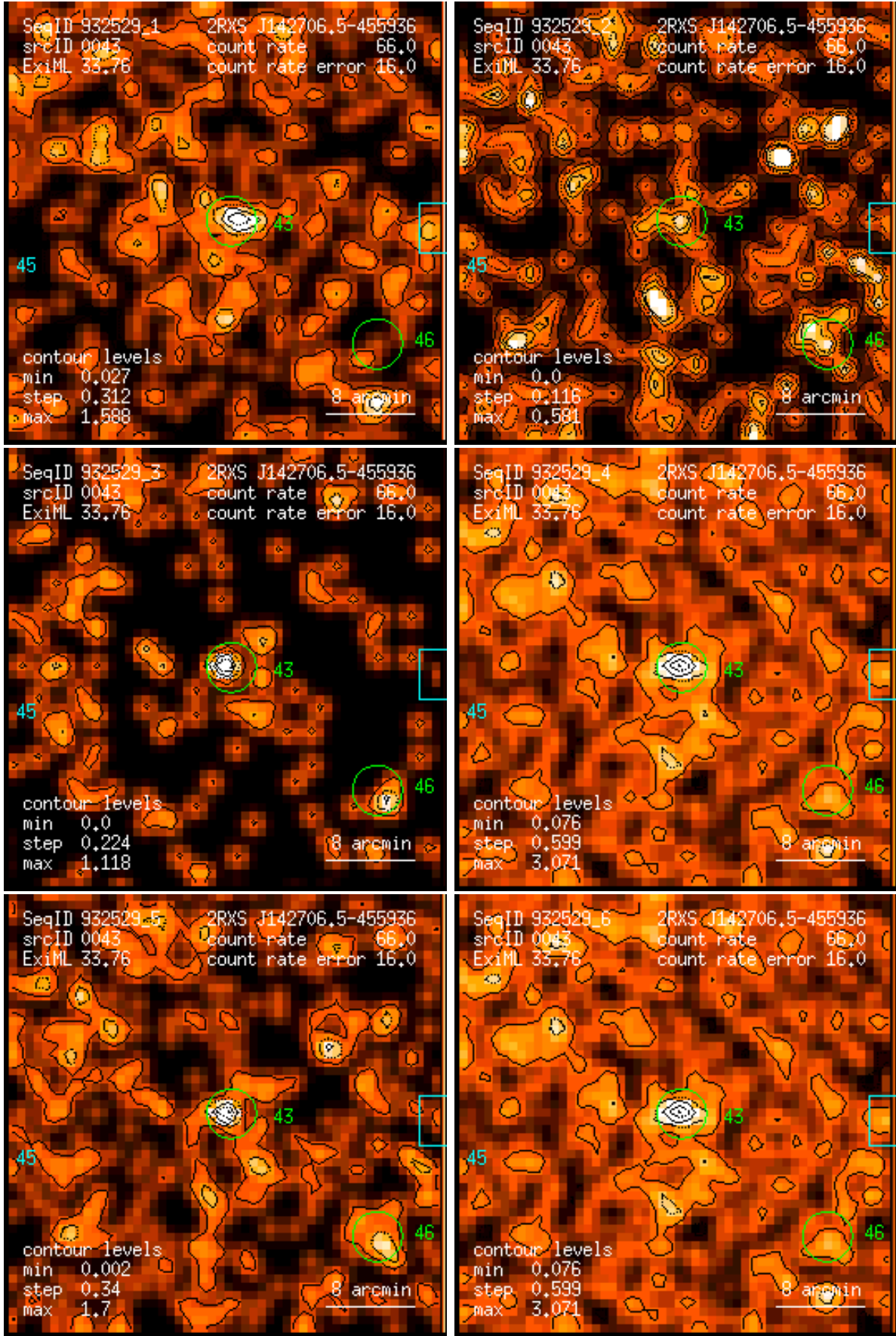
Figure 43: RASS 932529: detection 0043: band rate images, Gaussian filter: (1) PSPC channels 11 – 41, (2) 52 – 90, (3) 91 – 201, (4) 11 – 235, (5) 52 – 201, (6) 11 – 201. Broad band rates in counts/ks. Band rate contour levels in counts/ks/arcmin 2 .
