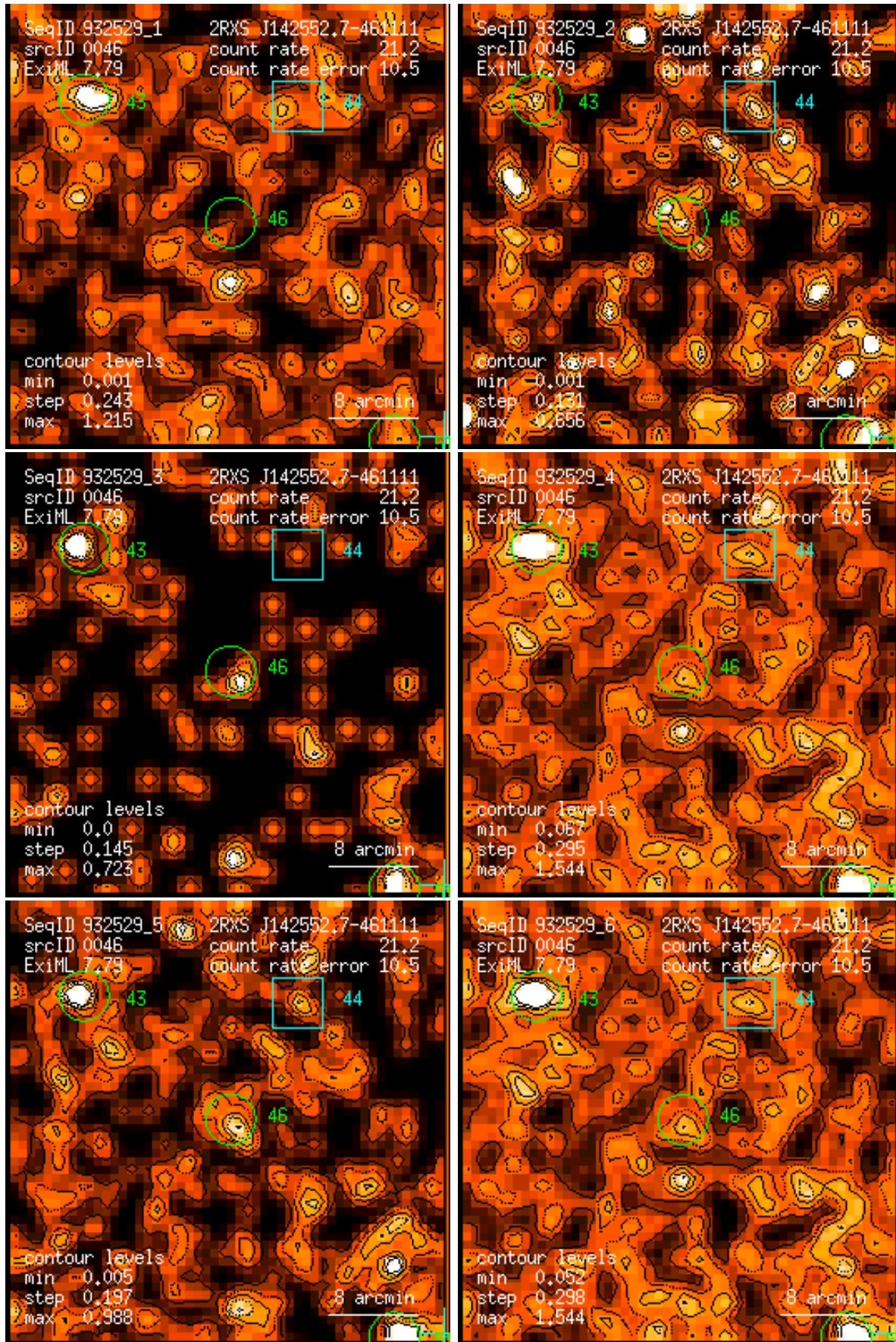
Figure 46: RASS 932529: detection 0046: band rate images, Gaussian filter: (1) PSPC channels 11 – 41, (2) 52 – 90, (3) 91 – 201, (4) 11 – 235, (5) 52 – 201, (6) 11 – 201. Broad band rates in counts/ks. Band rate contour levels in counts/ks/arcmin 2 .
