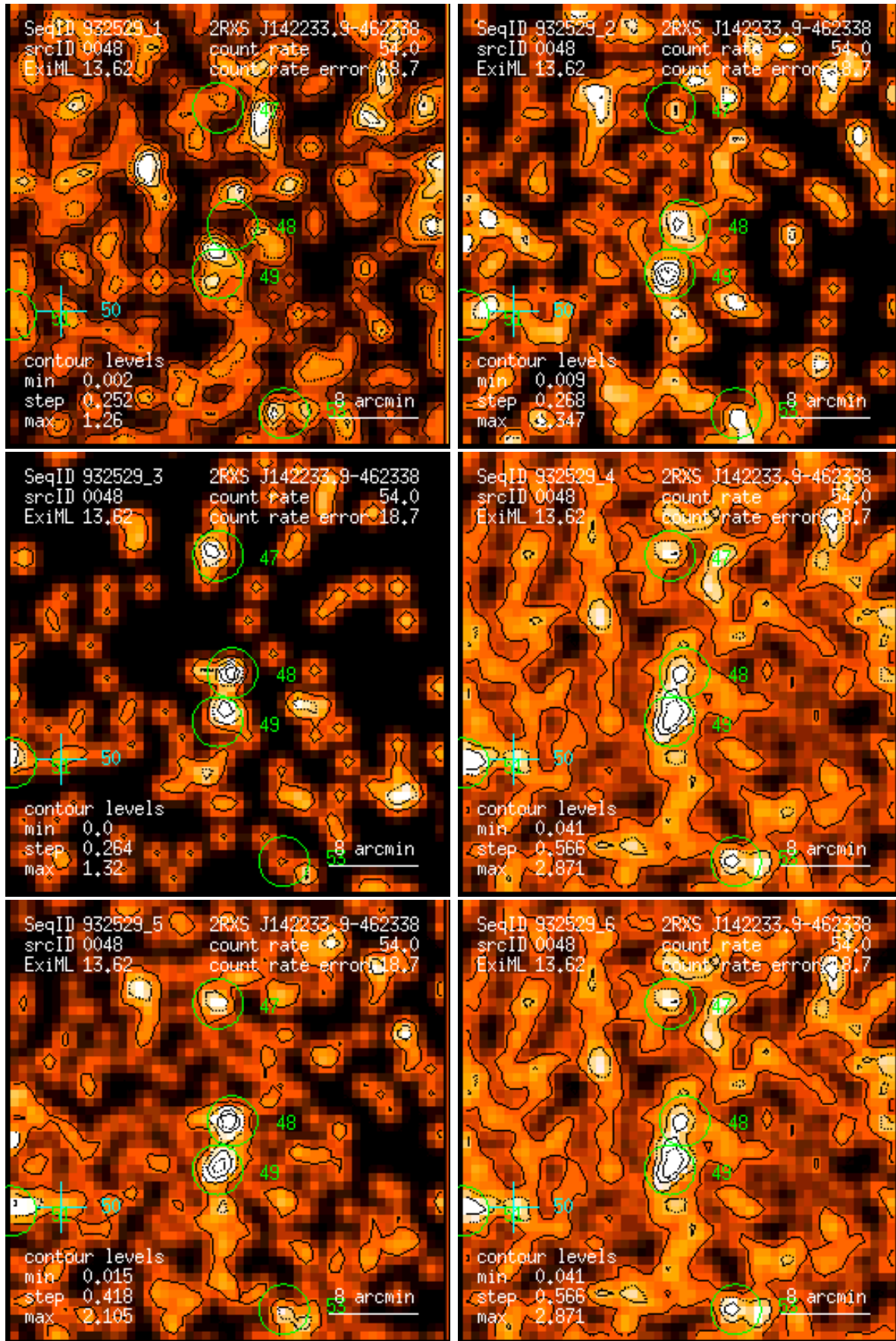
Figure 48: RASS 932529: detection 0048: band rate images, Gaussian filter: (1) PSPC channels 11 – 41, (2) 52 – 90, (3) 91 – 201, (4) 11 – 235, (5) 52 – 201, (6) 11 – 201. Broad band rates in counts/ks. Band rate contour levels in counts/ks/arcmin 2 .
