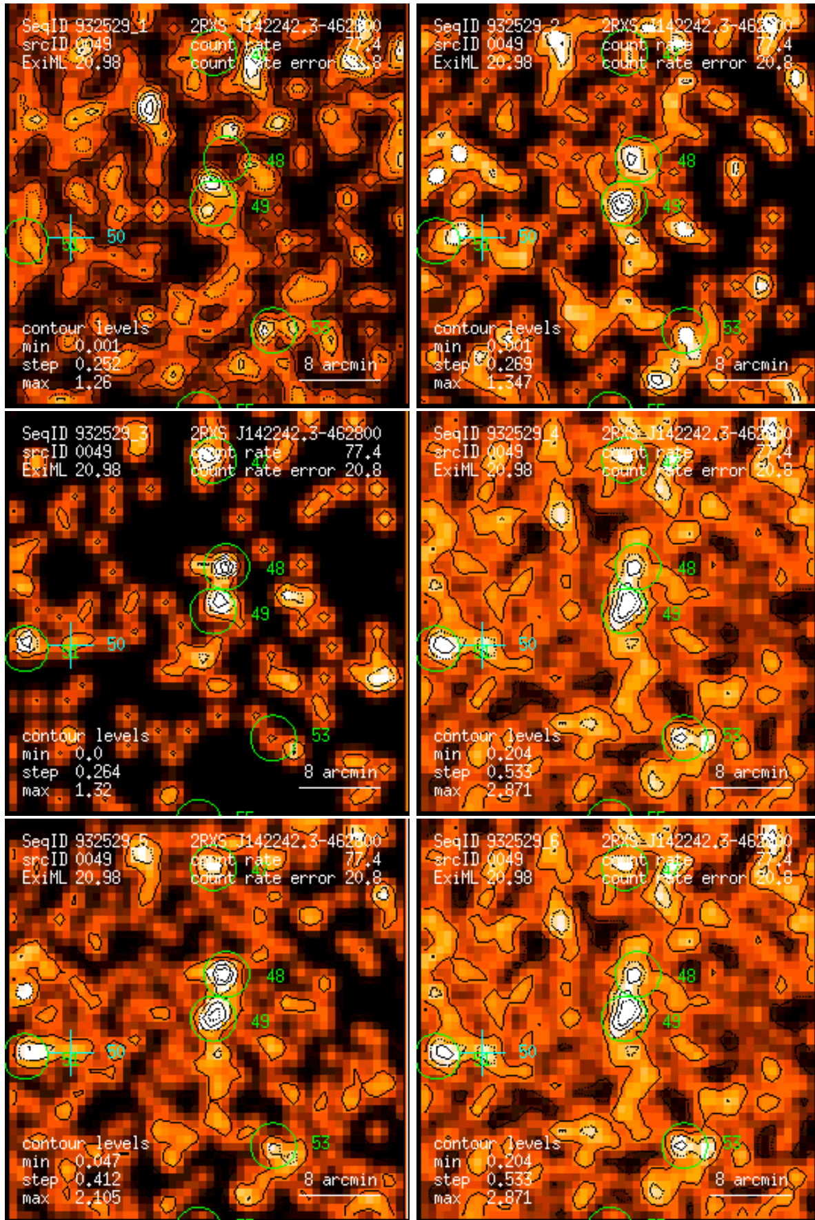
Figure 49: RASS 932529: detection 0049: band rate images, Gaussian filter: (1) PSPC channels 11 – 41, (2) 52 – 90, (3) 91 – 201, (4) 11 – 235, (5) 52 – 201, (6) 11 – 201. Broad band rates in counts/ks. Band rate contour levels in counts/ks/arcmin 2 .
