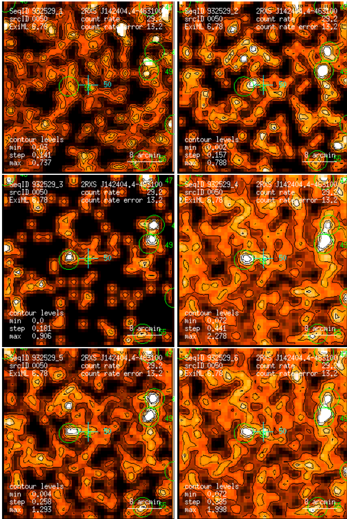
Figure 50: RASS 932529: detection 0050: band rate images, Gaussian filter: (1) PSPC channels 11 – 41, (2) 52 – 90, (3) 91 – 201, (4) 11 – 235, (5) 52 – 201, (6) 11 – 201. Broad band rates in counts/ks. Band rate contour levels in counts/ks/arcmin 2 .
