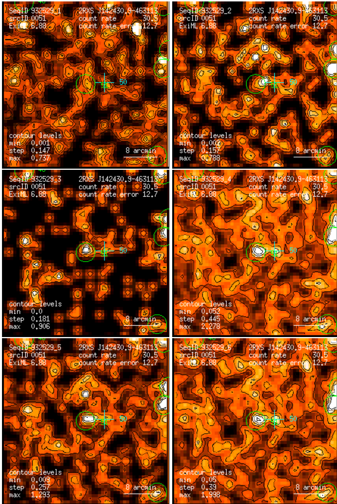
Figure 51: RASS 932529: detection 0051: band rate images, Gaussian filter: (1) PSPC channels 11 – 41, (2) 52 – 90, (3) 91 – 201, (4) 11 – 235, (5) 52 – 201, (6) 11 – 201. Broad band rates in counts/ks. Band rate contour levels in counts/ks/arcmin 2 .
