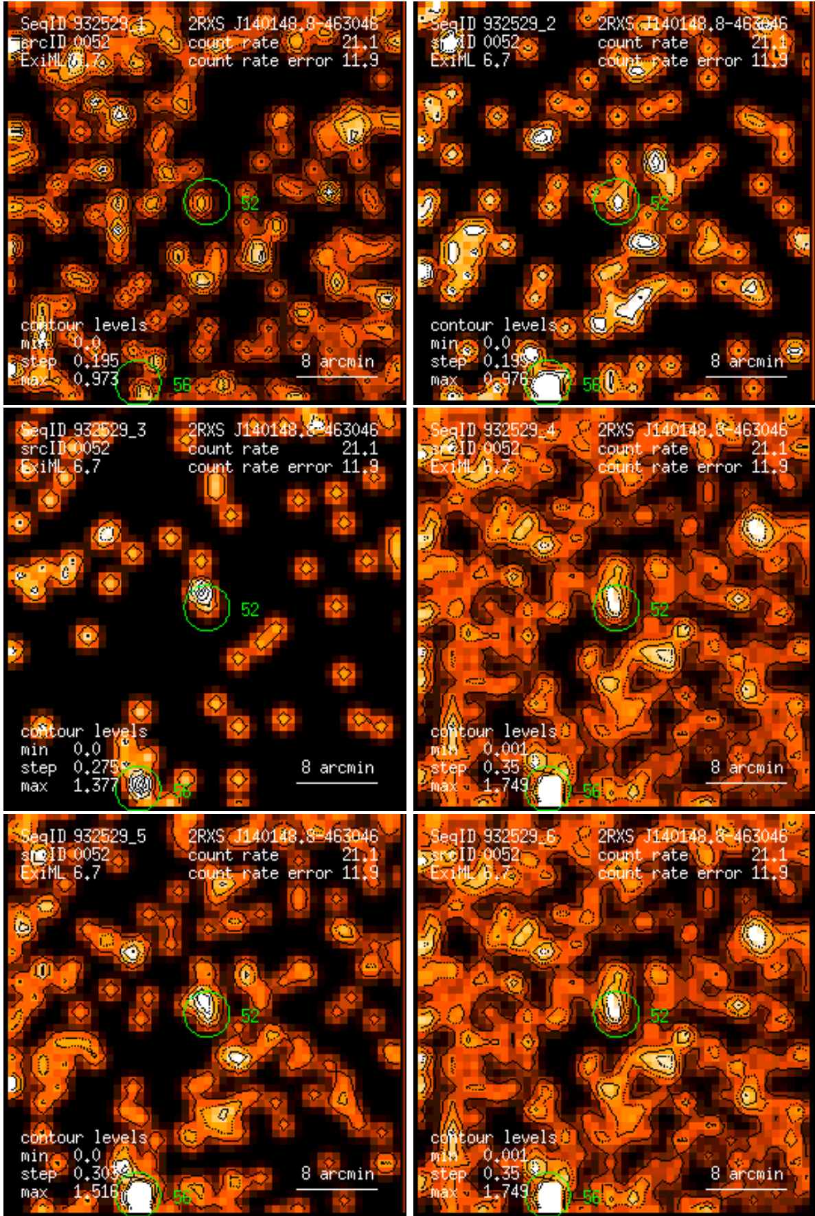
Figure 52: RASS 932529: detection 0052: band rate images, Gaussian filter: (1) PSPC channels 11 – 41, (2) 52 – 90, (3) 91 – 201, (4) 11 – 235, (5) 52 – 201, (6) 11 – 201. Broad band rates in counts/ks. Band rate contour levels in counts/ks/arcmin 2 .
