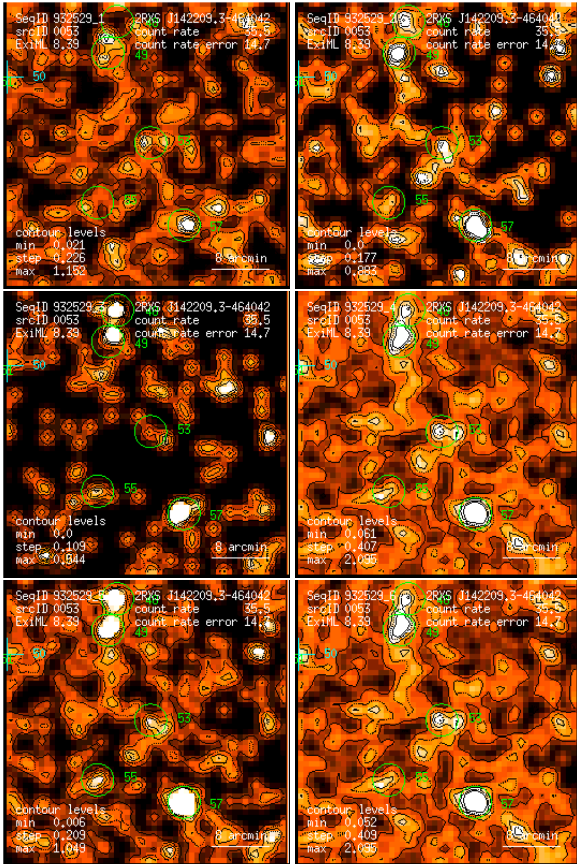
Figure 53: RASS 932529: detection 0053: band rate images, Gaussian filter: (1) PSPC channels 11 – 41, (2) 52 – 90, (3) 91 – 201, (4) 11 – 235, (5) 52 – 201, (6) 11 – 201. Broad band rates in counts/ks. Band rate contour levels in counts/ks/arcmin 2 .
