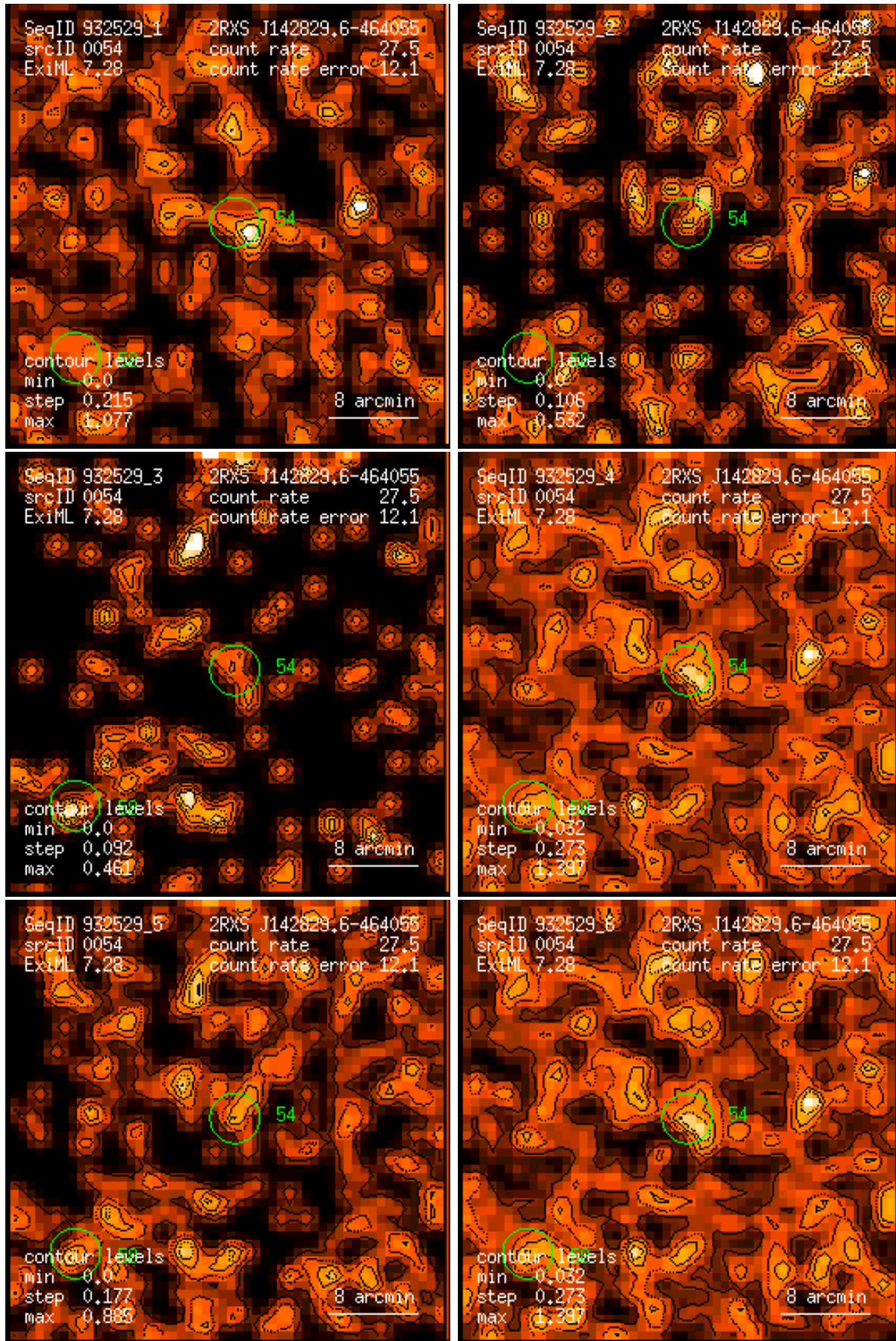
Figure 54: RASS 932529: detection 0054: band rate images, Gaussian filter: (1) PSPC channels 11 – 41, (2) 52 – 90, (3) 91 – 201, (4) 11 – 235, (5) 52 – 201, (6) 11 – 201. Broad band rates in counts/ks. Band rate contour levels in counts/ks/arcmin 2 .
