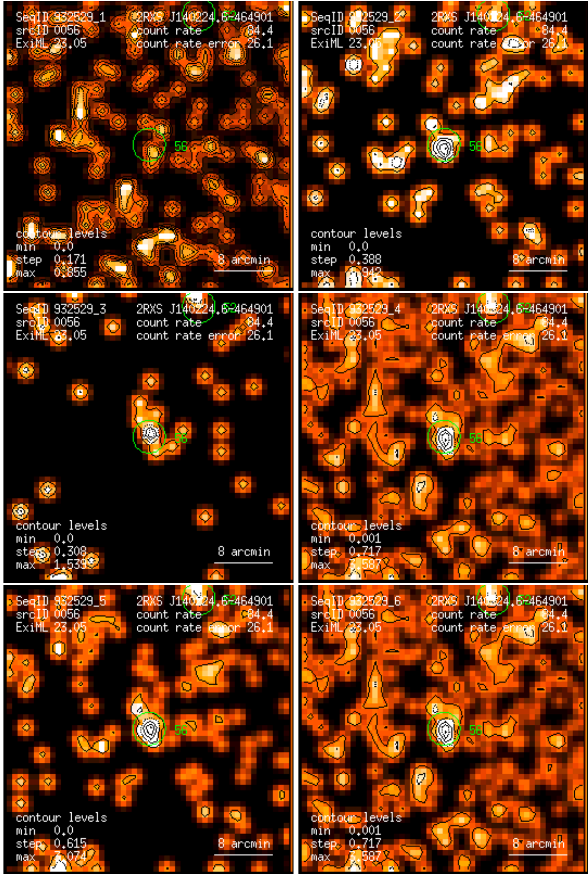
Figure 56: RASS 932529: detection 0056: band rate images, Gaussian filter: (1) PSPC channels 11 – 41, (2) 52 – 90, (3) 91 – 201, (4) 11 – 235, (5) 52 – 201, (6) 11 – 201. Broad band rates in counts/ks. Band rate contour levels in counts/ks/arcmin 2 .
