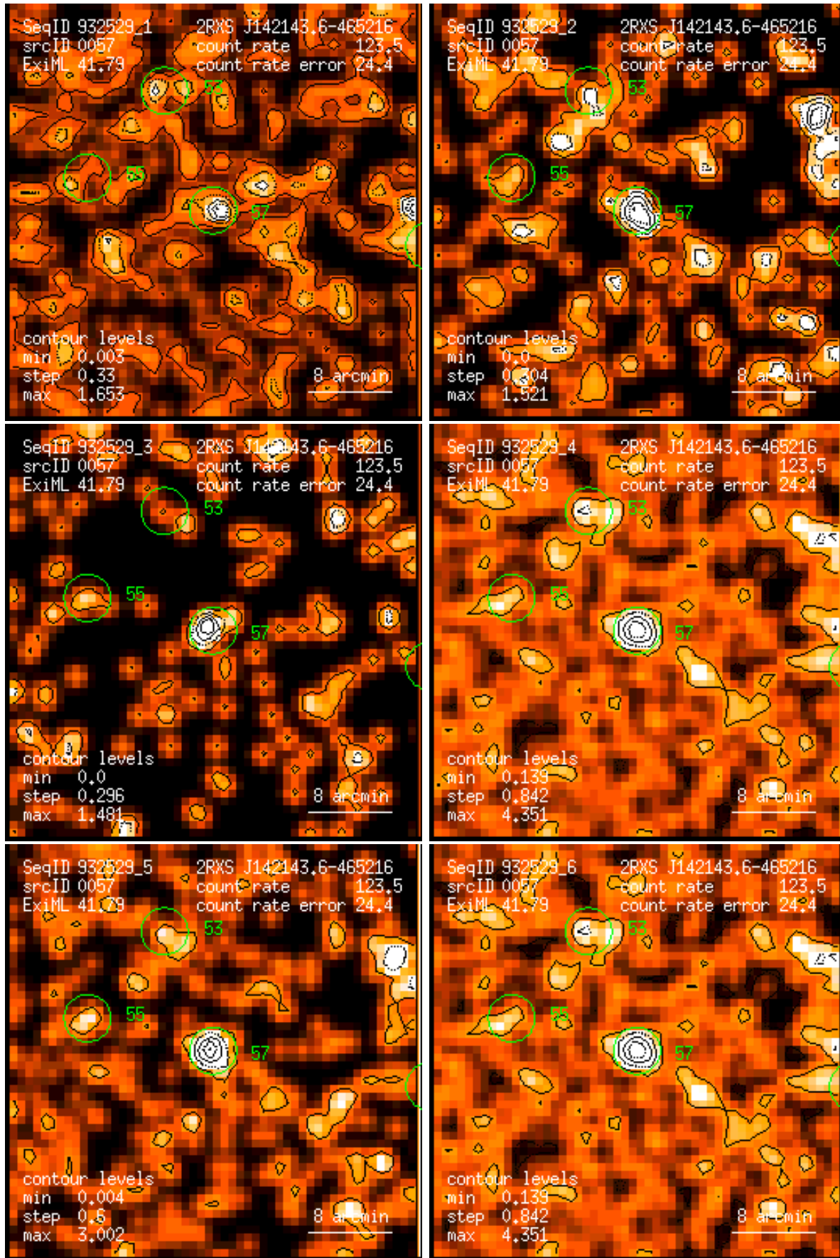
Figure 57: RASS 932529: detection 0057: band rate images, Gaussian filter: (1) PSPC channels 11 – 41, (2) 52 – 90, (3) 91 – 201, (4) 11 – 235, (5) 52 – 201, (6) 11 – 201. Broad band rates in counts/ks. Band rate contour levels in counts/ks/arcmin 2 .
