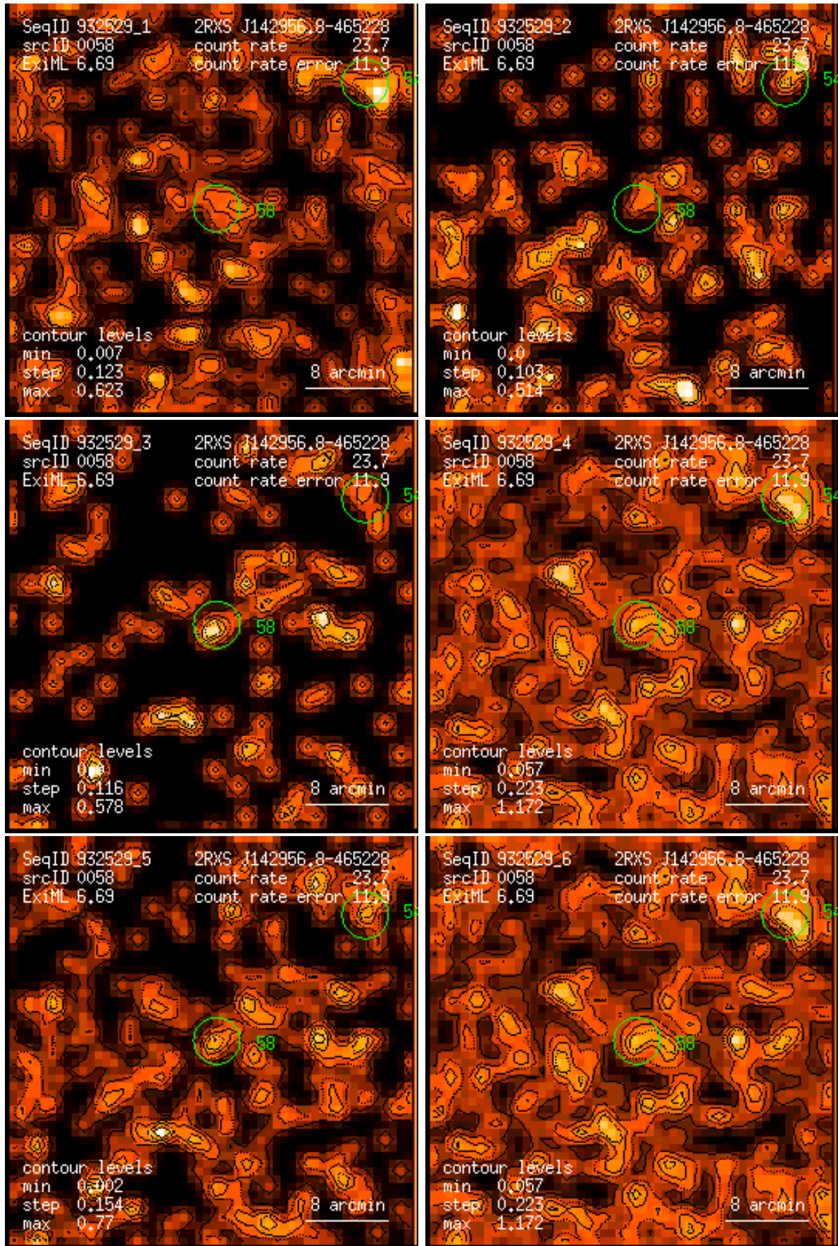
Figure 58: RASS 932529: detection 0058: band rate images, Gaussian filter: (1) PSPC channels 11 – 41, (2) 52 – 90, (3) 91 – 201, (4) 11 – 235, (5) 52 – 201, (6) 11 – 201. Broad band rates in counts/ks. Band rate contour levels in counts/ks/arcmin 2 .
