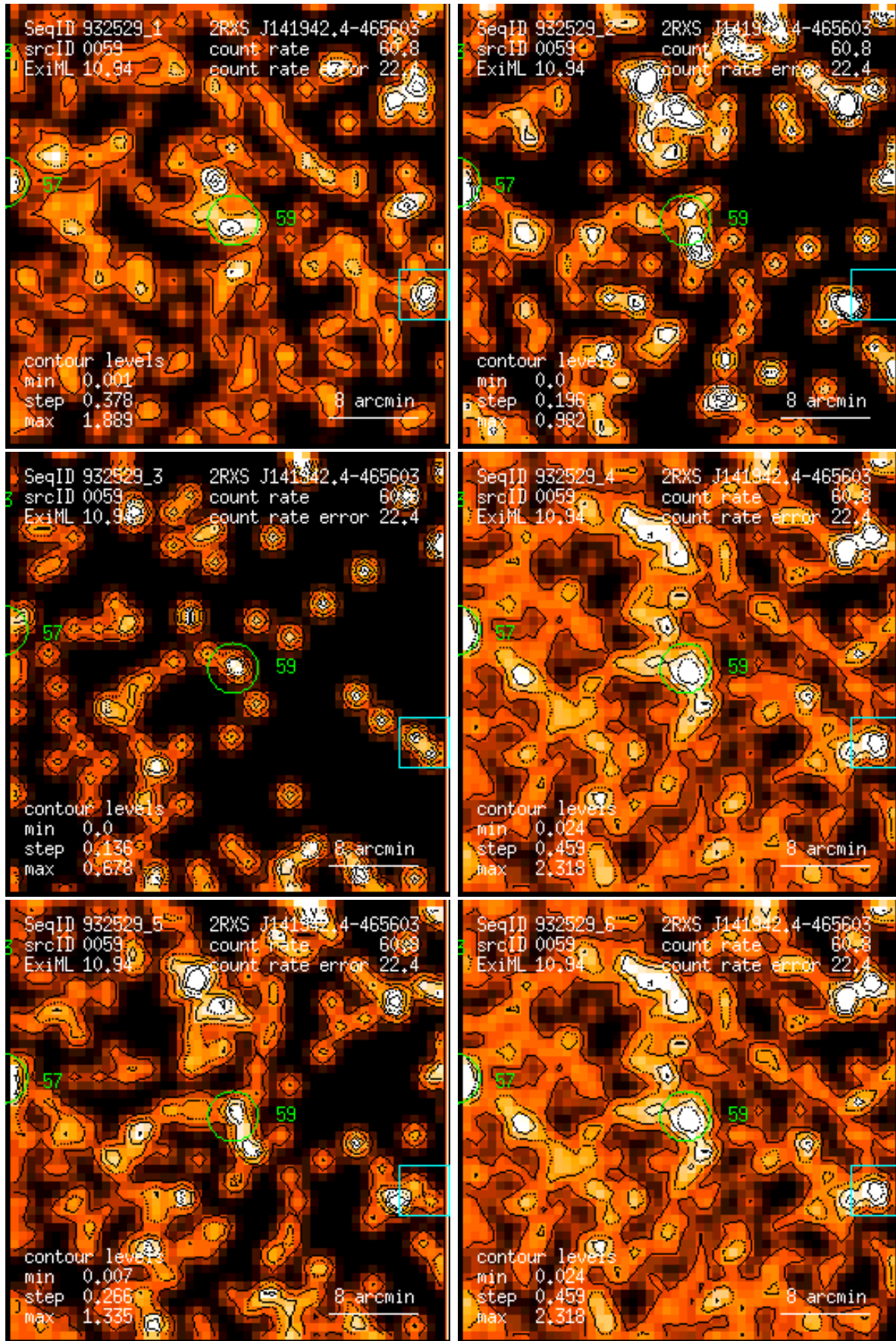
Figure 59: RASS 932529: detection 0059: band rate images, Gaussian filter: (1) PSPC channels 11 – 41, (2) 52 – 90, (3) 91 – 201, (4) 11 – 235, (5) 52 – 201, (6) 11 – 201. Broad band rates in counts/ks. Band rate contour levels in counts/ks/arcmin 2 .
