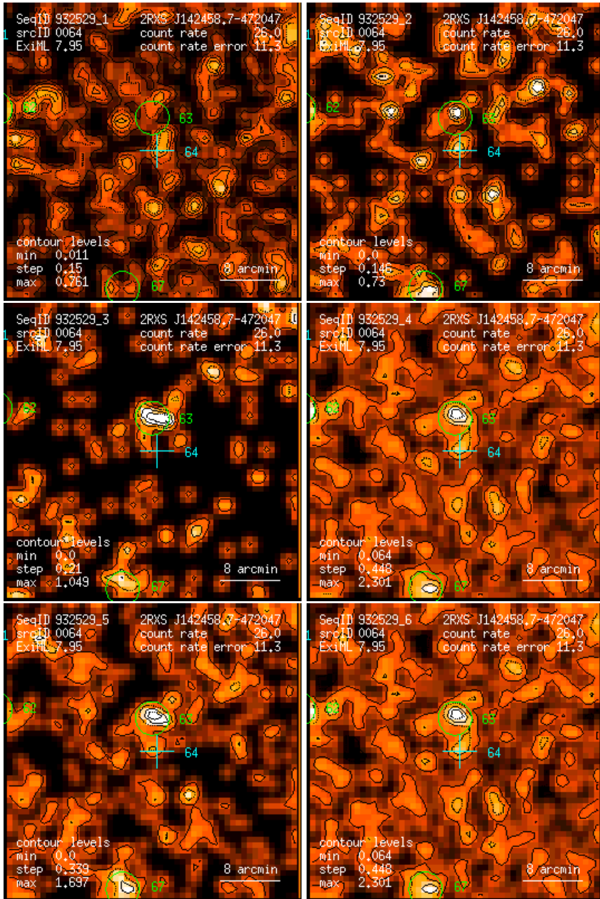
Figure 64: RASS 932529: detection 0064: band rate images, Gaussian filter: (1) PSPC channels 11 – 41, (2) 52 – 90, (3) 91 – 201, (4) 11 – 235, (5) 52 – 201, (6) 11 – 201. Broad band rates in counts/ks. Band rate contour levels in counts/ks/arcmin 2 .
