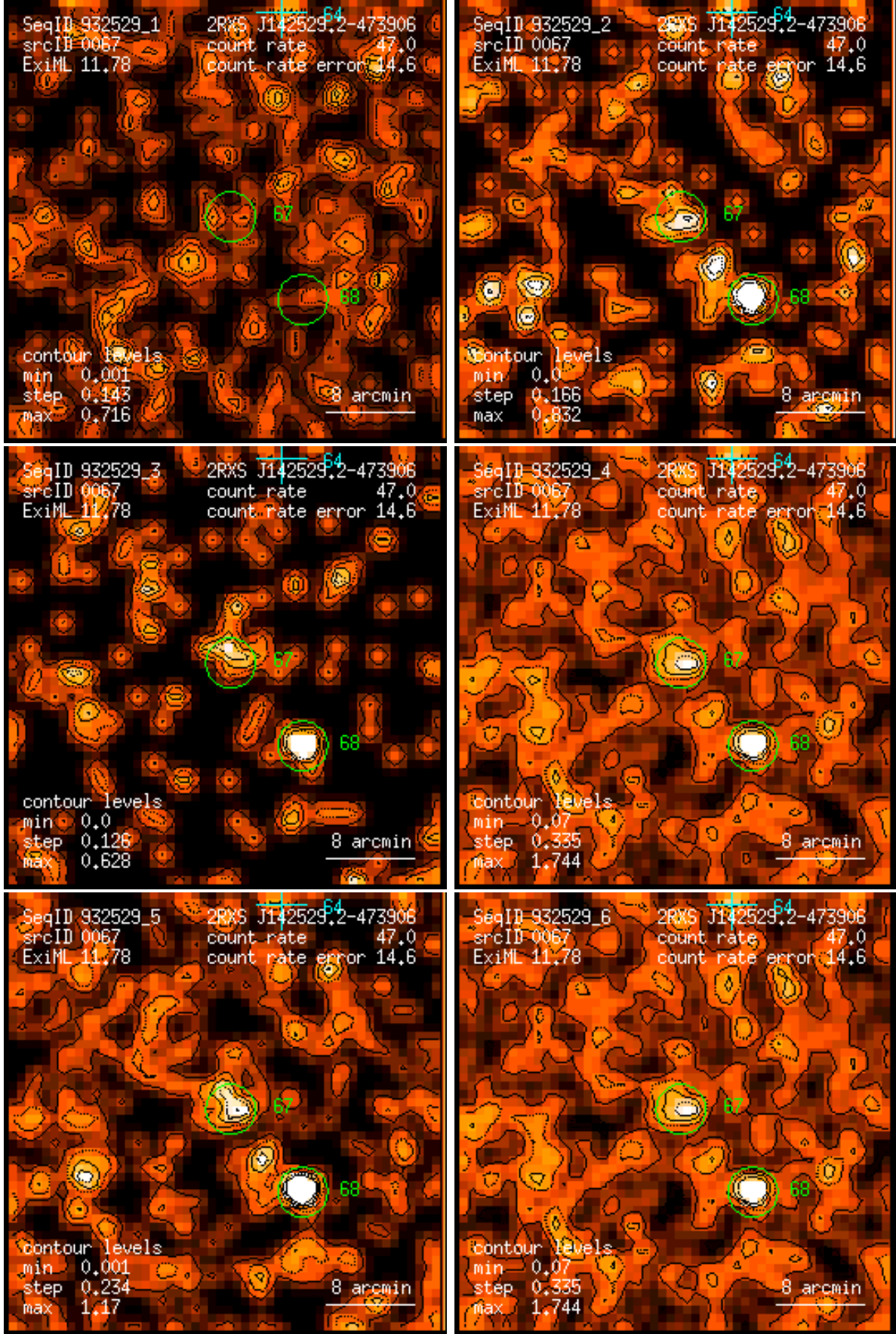
Figure 67: RASS 932529: detection 0067: band rate images, Gaussian filter: (1) PSPC channels 11 – 41, (2) 52 – 90, (3) 91 – 201, (4) 11 – 235, (5) 52 – 201, (6) 11 – 201. Broad band rates in counts/ks. Band rate contour levels in counts/ks/arcmin 2 .
