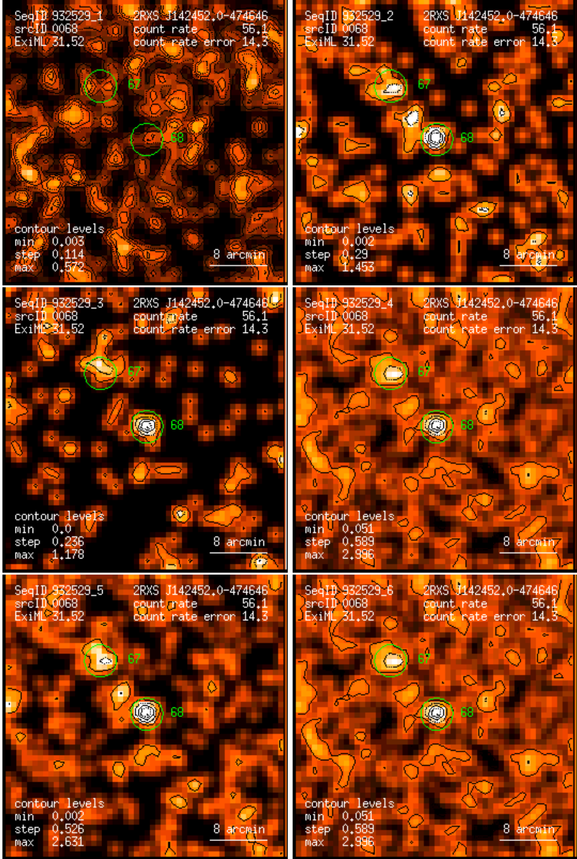
Figure 68: RASS 932529: detection 0068: band rate images, Gaussian filter: (1) PSPC channels 11 – 41, (2) 52 – 90, (3) 91 – 201, (4) 11 – 235, (5) 52 – 201, (6) 11 – 201. Broad band rates in counts/ks. Band rate contour levels in counts/ks/arcmin 2 .
