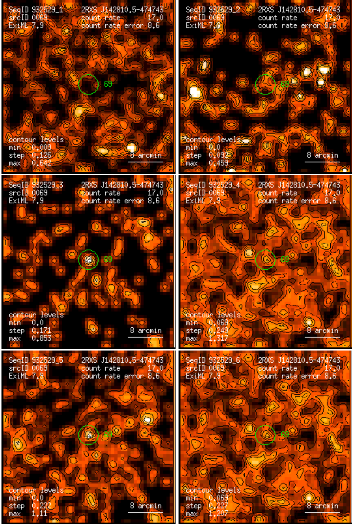
Figure 69: RASS 932529: detection 0069: band rate images, Gaussian filter: (1) PSPC channels 11 – 41, (2) 52 – 90, (3) 91 – 201, (4) 11 – 235, (5) 52 – 201, (6) 11 – 201. Broad band rates in counts/ks. Band rate contour levels in counts/ks/arcmin 2 .
