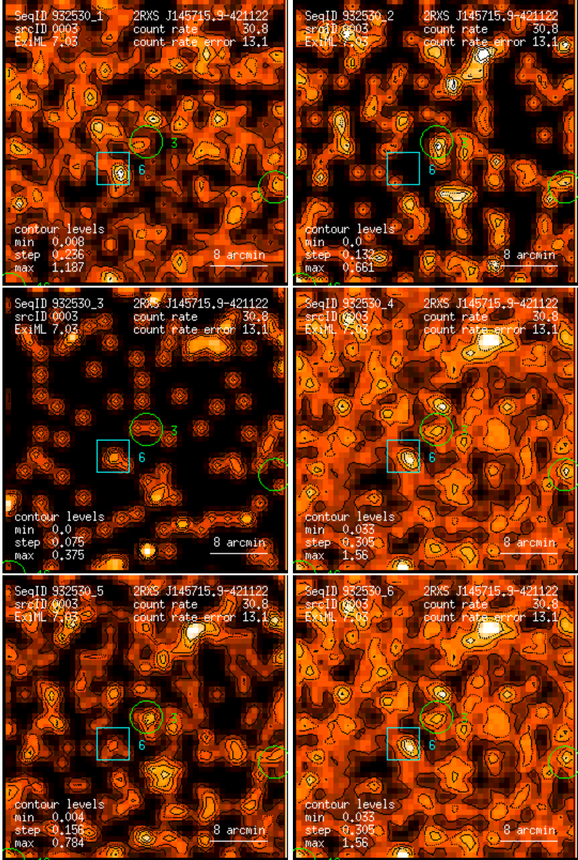
Figure 3: RASS 932530: detection 0003: band rate images, Gaussian filter: (1) PSPC channels 11 – 41, (2) 52 – 90, (3) 91 – 201, (4) 11 – 235, (5) 52 – 201, (6) 11 – 201. Broad band rates in counts/ks. Band rate contour levels in counts/ks/arcmin 2 .
