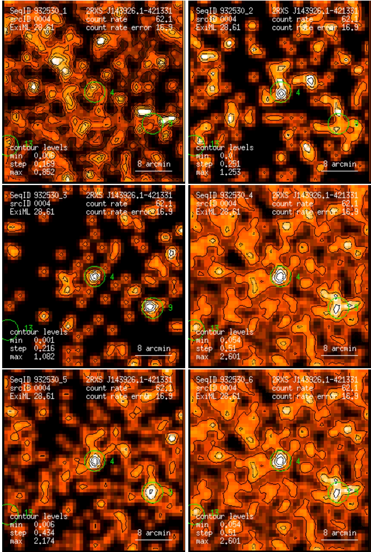
Figure 4: RASS 932530: detection 0004: band rate images, Gaussian filter: (1) PSPC channels 11 – 41, (2) 52 – 90, (3) 91 – 201, (4) 11 – 235, (5) 52 – 201, (6) 11 – 201. Broad band rates in counts/ks. Band rate contour levels in counts/ks/arcmin 2 .
