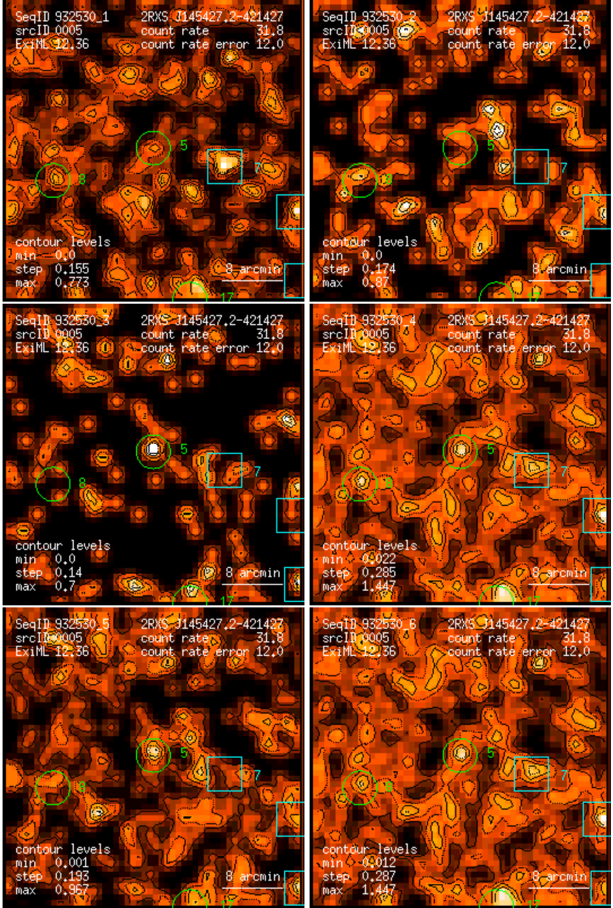
Figure 5: RASS 932530: detection 0005: band rate images, Gaussian filter: (1) PSPC channels 11 – 41, (2) 52 – 90, (3) 91 – 201, (4) 11 – 235, (5) 52 – 201, (6) 11 – 201. Broad band rates in counts/ks. Band rate contour levels in counts/ks/arcmin 2 .
