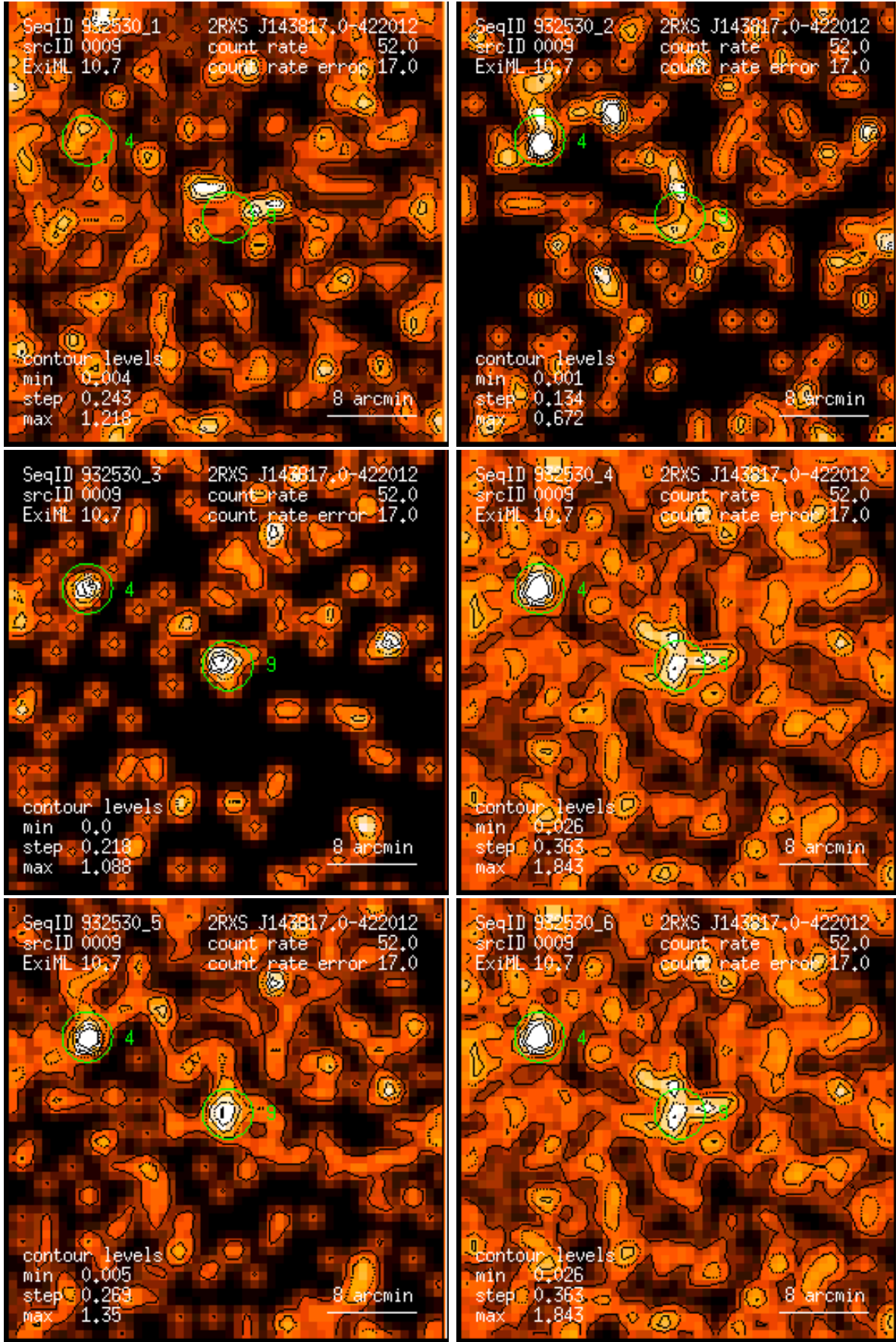
Figure 9: RASS 932530: detection 0009: band rate images, Gaussian filter: (1) PSPC channels 11 – 41, (2) 52 – 90, (3) 91 – 201, (4) 11 – 235, (5) 52 – 201, (6) 11 – 201. Broad band rates in counts/ks. Band rate contour levels in counts/ks/arcmin 2 .
