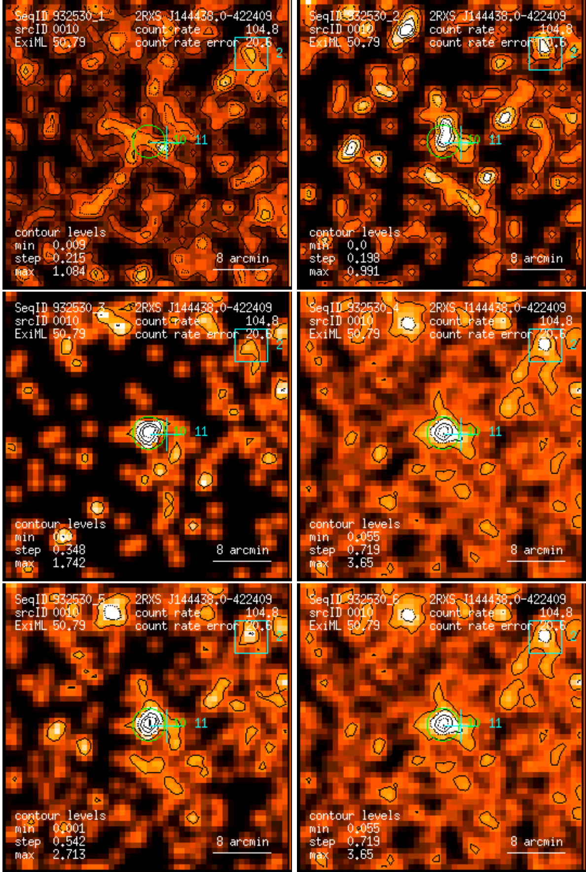
Figure 10: RASS 932530: detection 0010: band rate images, Gaussian filter: (1) PSPC channels 11 – 41, (2) 52 – 90, (3) 91 – 201, (4) 11 – 235, (5) 52 – 201, (6) 11 – 201. Broad band rates in counts/ks. Band rate contour levels in counts/ks/arcmin 2 .
