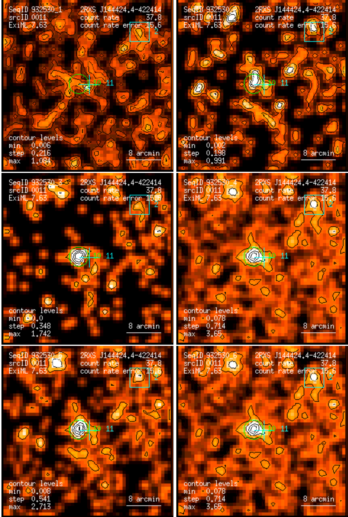
Figure 11: RASS 932530: detection 0011: band rate images, Gaussian filter: (1) PSPC channels 11 – 41, (2) 52 – 90, (3) 91 – 201, (4) 11 – 235, (5) 52 – 201, (6) 11 – 201. Broad band rates in counts/ks. Band rate contour levels in counts/ks/arcmin 2 .
