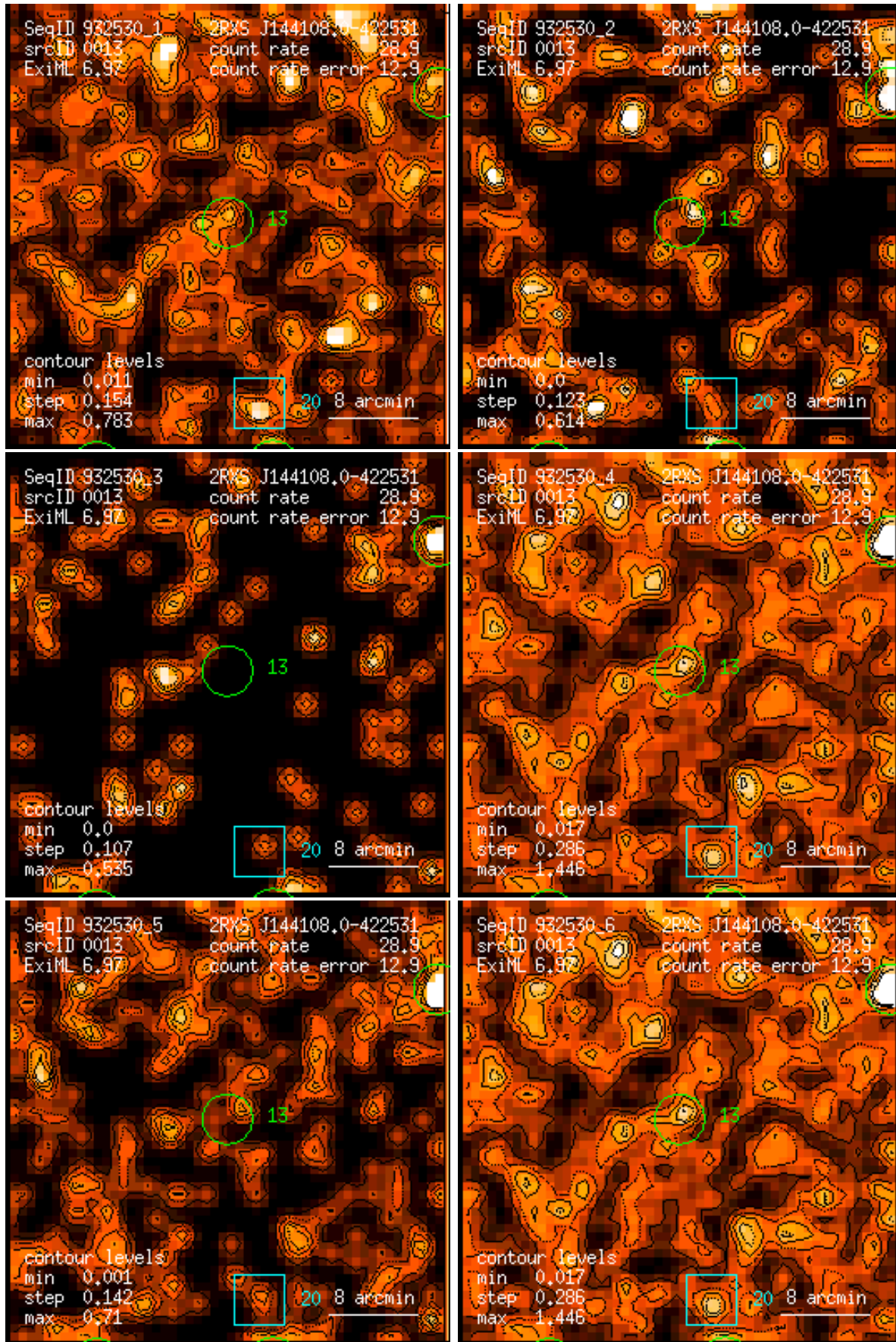
Figure 13: RASS 932530: detection 0013: band rate images, Gaussian filter: (1) PSPC channels 11 – 41, (2) 52 – 90, (3) 91 – 201, (4) 11 – 235, (5) 52 – 201, (6) 11 – 201. Broad band rates in counts/ks. Band rate contour levels in counts/ks/arcmin 2 .
