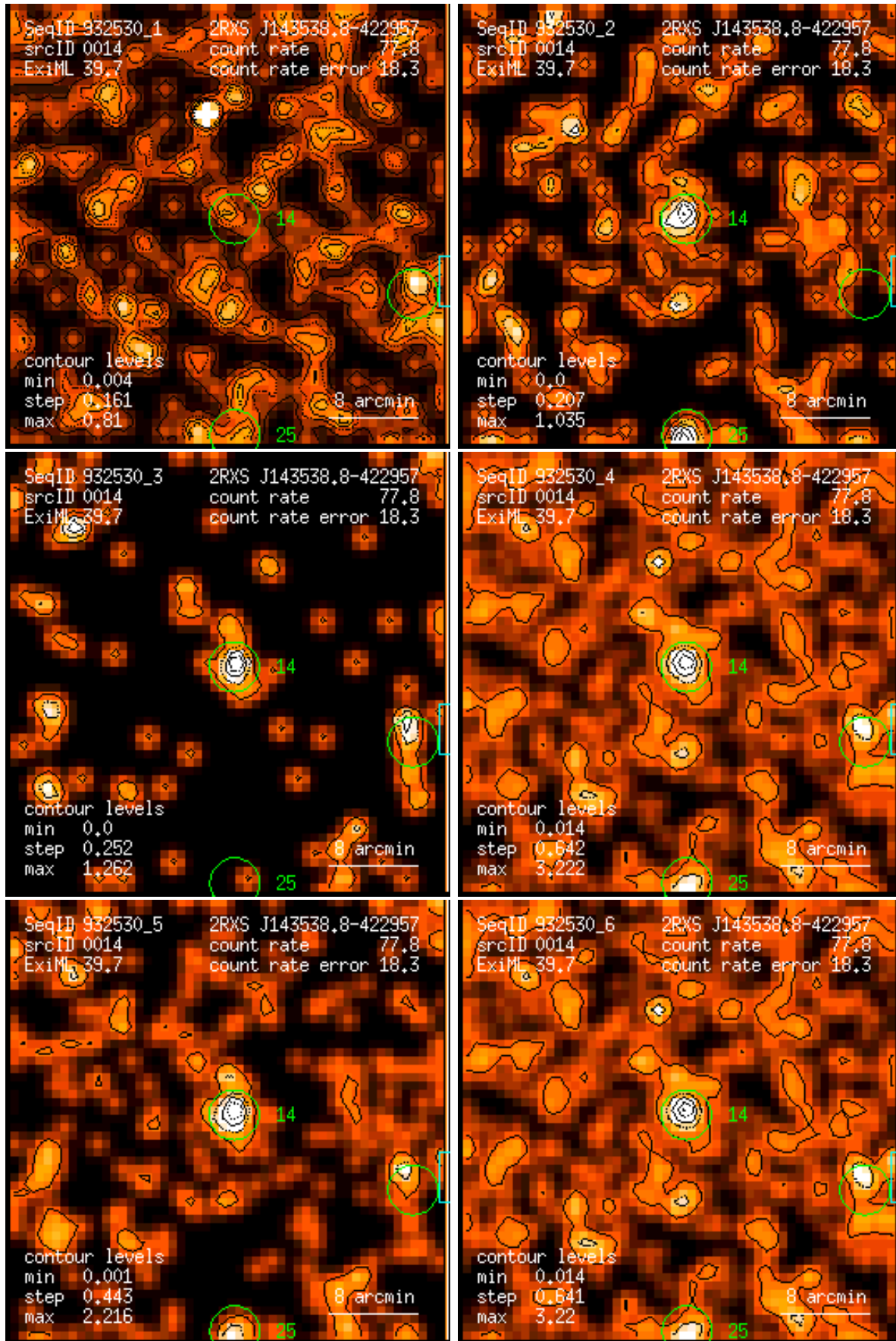
Figure 14: RASS 932530: detection 0014: band rate images, Gaussian filter: (1) PSPC channels 11 – 41, (2) 52 – 90, (3) 91 – 201, (4) 11 – 235, (5) 52 – 201, (6) 11 – 201. Broad band rates in counts/ks. Band rate contour levels in counts/ks/arcmin 2 .
