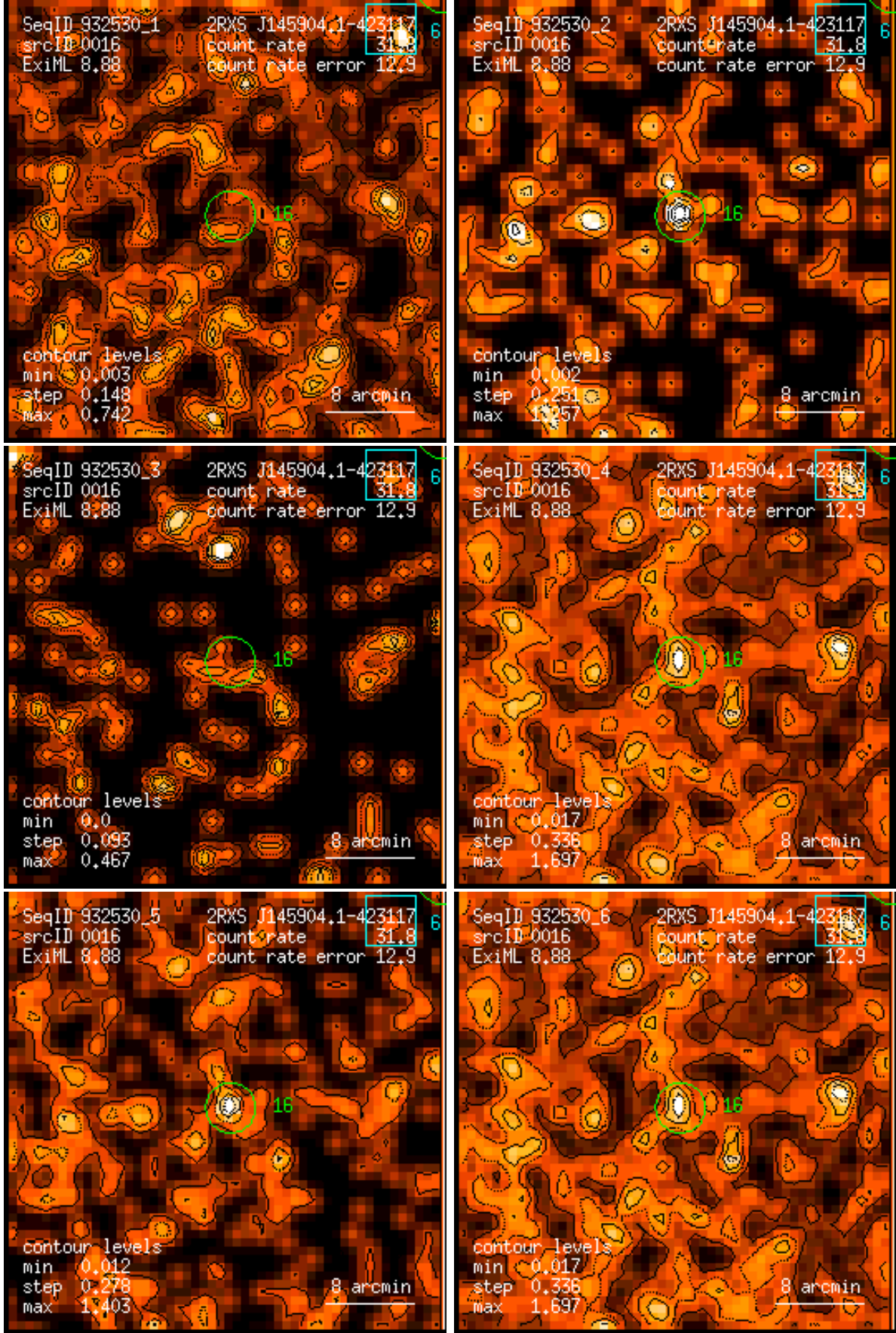
Figure 16: RASS 932530: detection 0016: band rate images, Gaussian filter: (1) PSPC channels 11 – 41, (2) 52 – 90, (3) 91 – 201, (4) 11 – 235, (5) 52 – 201, (6) 11 – 201. Broad band rates in counts/ks. Band rate contour levels in counts/ks/arcmin 2 .
