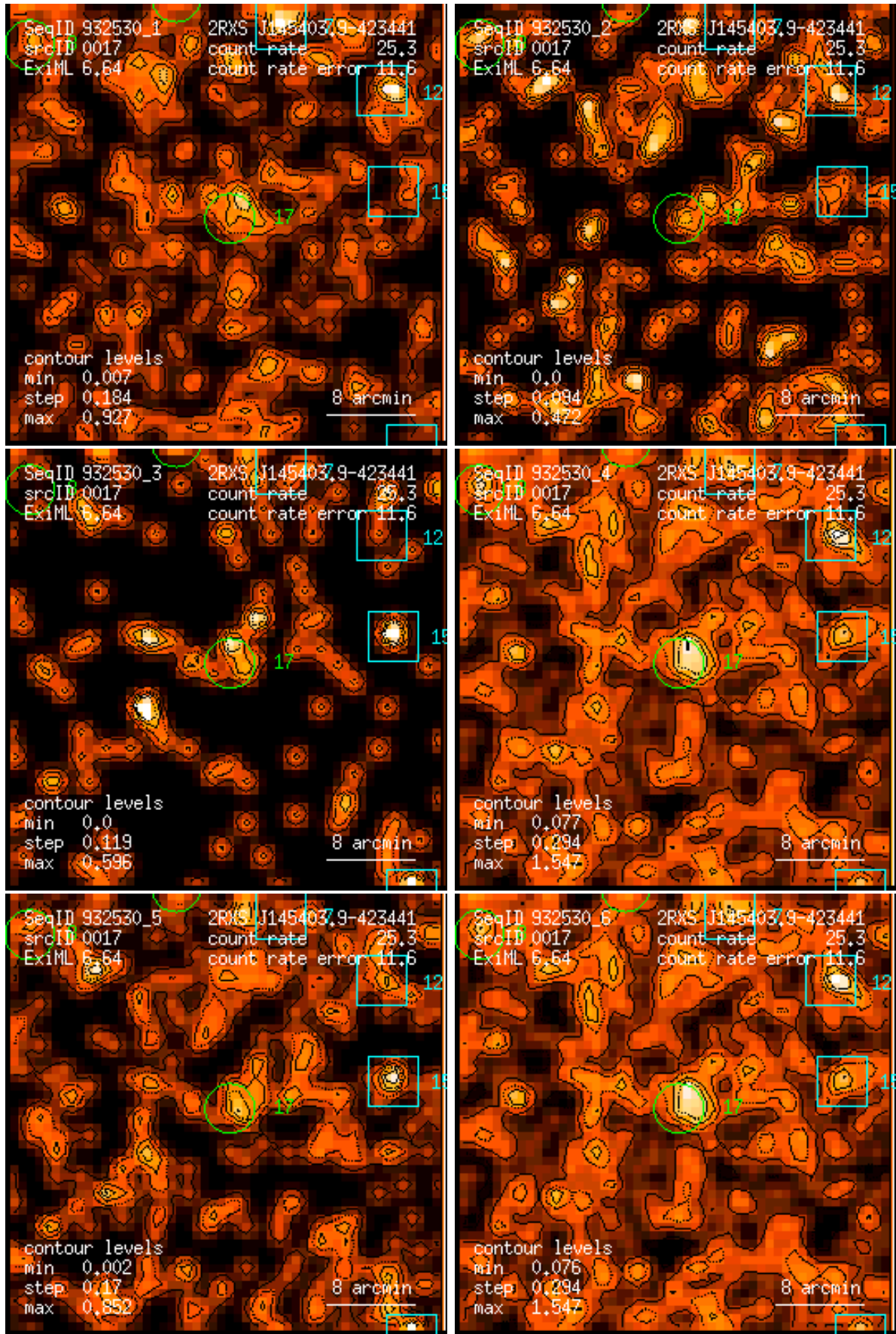
Figure 17: RASS 932530: detection 0017: band rate images, Gaussian filter: (1) PSPC channels 11 – 41, (2) 52 – 90, (3) 91 – 201, (4) 11 – 235, (5) 52 – 201, (6) 11 – 201. Broad band rates in counts/ks. Band rate contour levels in counts/ks/arcmin 2 .
