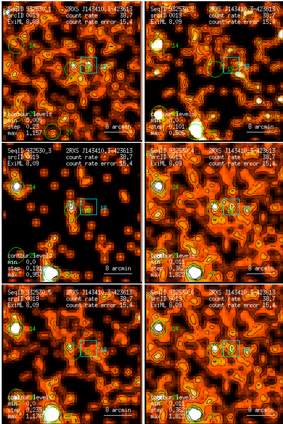
Figure 19: RASS 932530: detection 0019: band rate images, Gaussian filter: (1) PSPC channels 11 – 41, (2) 52 – 90, (3) 91 – 201, (4) 11 – 235, (5) 52 – 201, (6) 11 – 201. Broad band rates in counts/ks. Band rate contour levels in counts/ks/arcmin 2 .
