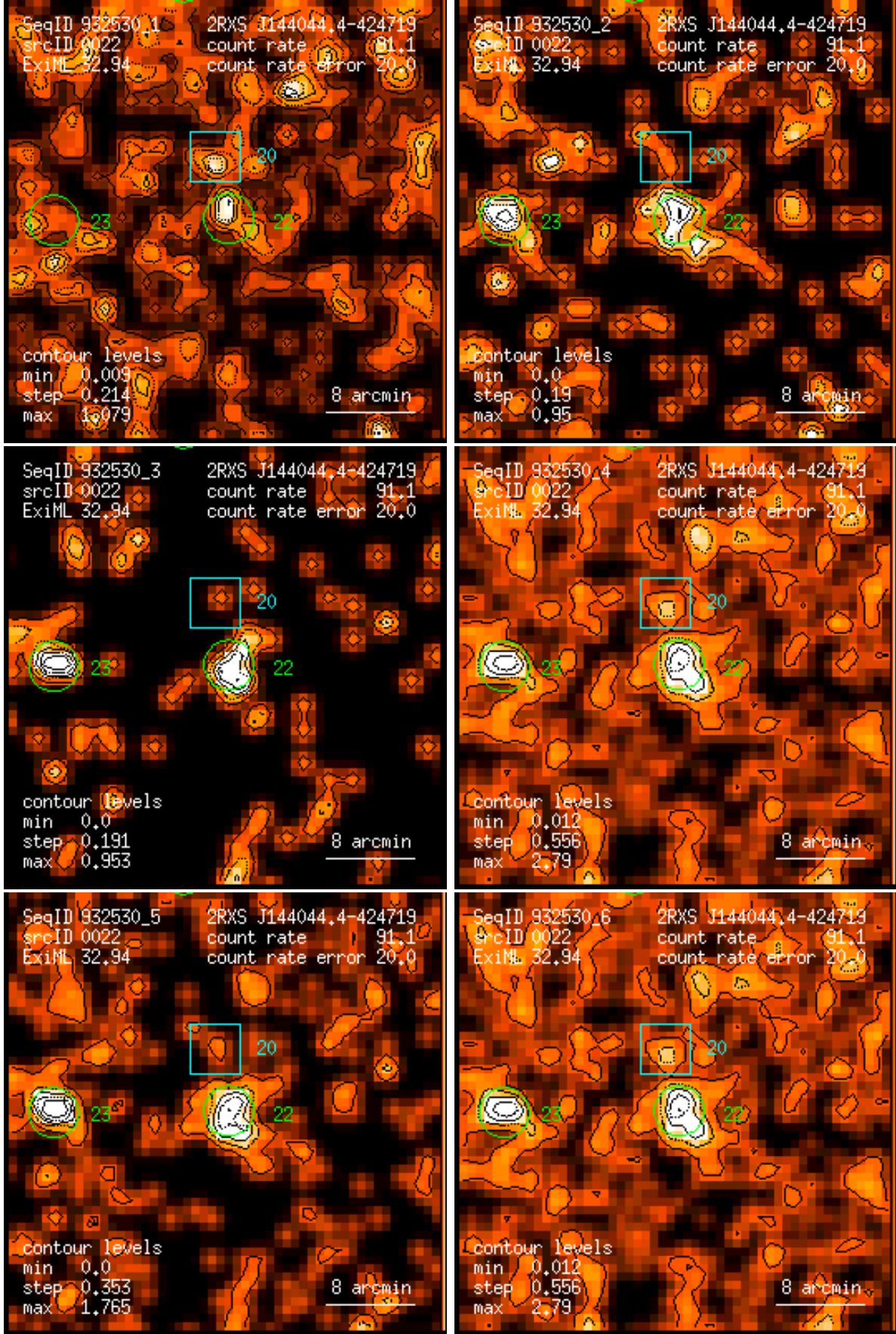
Figure 22: RASS 932530: detection 0022: band rate images, Gaussian filter: (1) PSPC channels 11 – 41, (2) 52 – 90, (3) 91 – 201, (4) 11 – 235, (5) 52 – 201, (6) 11 – 201. Broad band rates in counts/ks. Band rate contour levels in counts/ks/arcmin 2 .
