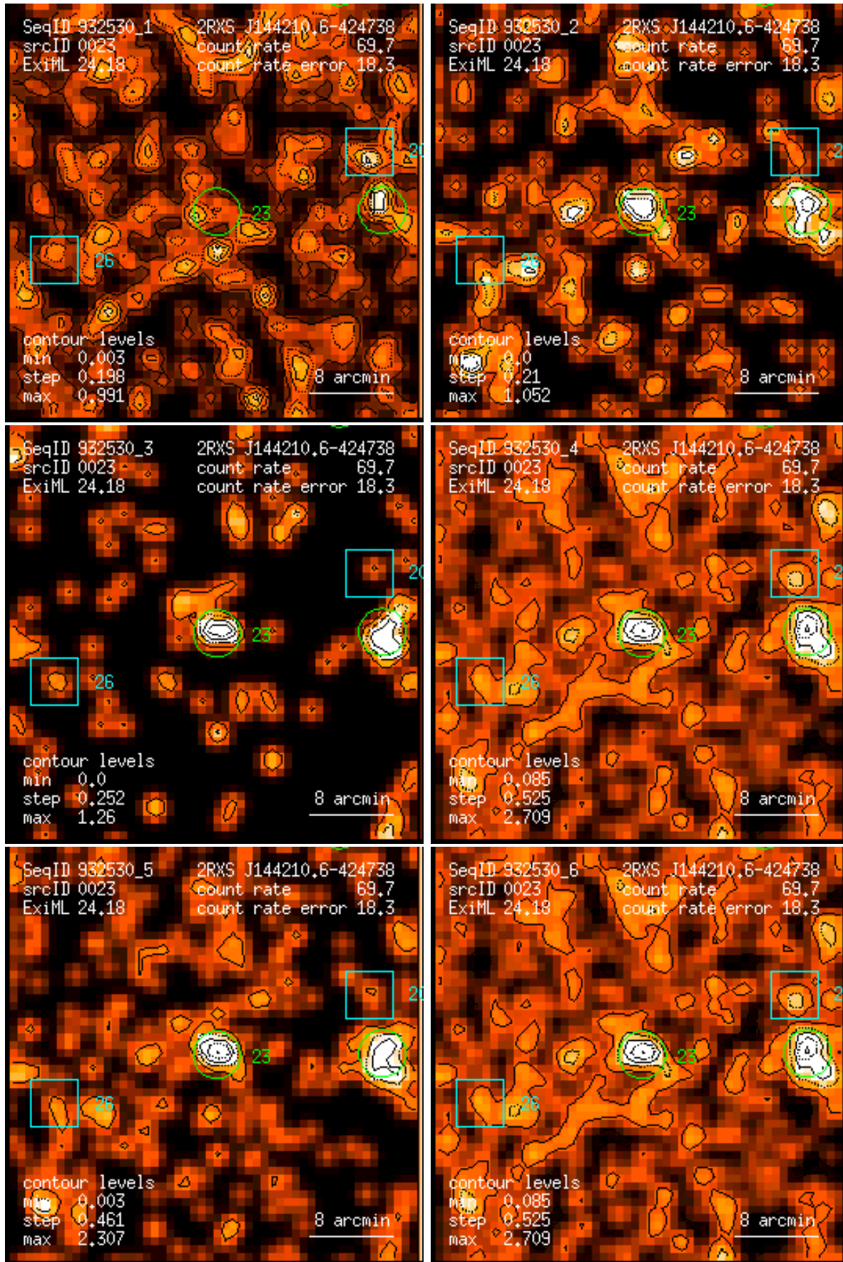
Figure 23: RASS 932530: detection 0023: band rate images, Gaussian filter: (1) PSPC channels 11 – 41, (2) 52 – 90, (3) 91 – 201, (4) 11 – 235, (5) 52 – 201, (6) 11 – 201. Broad band rates in counts/ks. Band rate contour levels in counts/ks/arcmin 2 .
