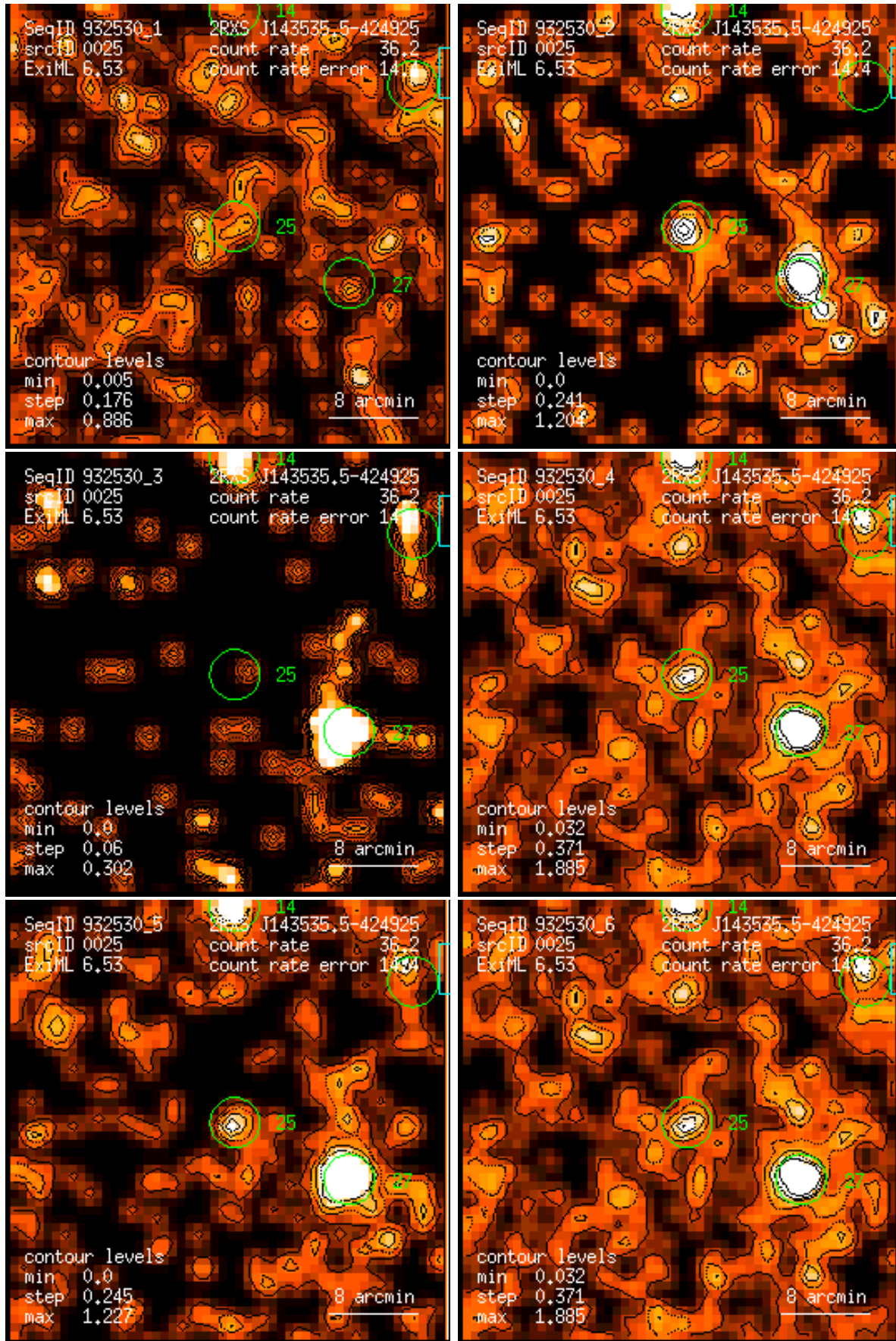
Figure 25: RASS 932530: detection 0025: band rate images, Gaussian filter: (1) PSPC channels 11 – 41, (2) 52 – 90, (3) 91 – 201, (4) 11 – 235, (5) 52 – 201, (6) 11 – 201. Broad band rates in counts/ks. Band rate contour levels in counts/ks/arcmin 2 .
