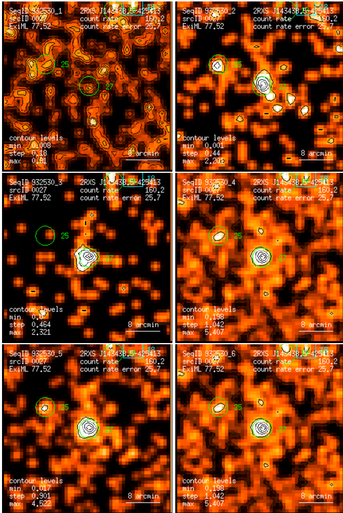
Figure 27: RASS 932530: detection 0027: band rate images, Gaussian filter: (1) PSPC channels 11 – 41, (2) 52 – 90, (3) 91 – 201, (4) 11 – 235, (5) 52 – 201, (6) 11 – 201. Broad band rates in counts/ks. Band rate contour levels in counts/ks/arcmin 2 .
