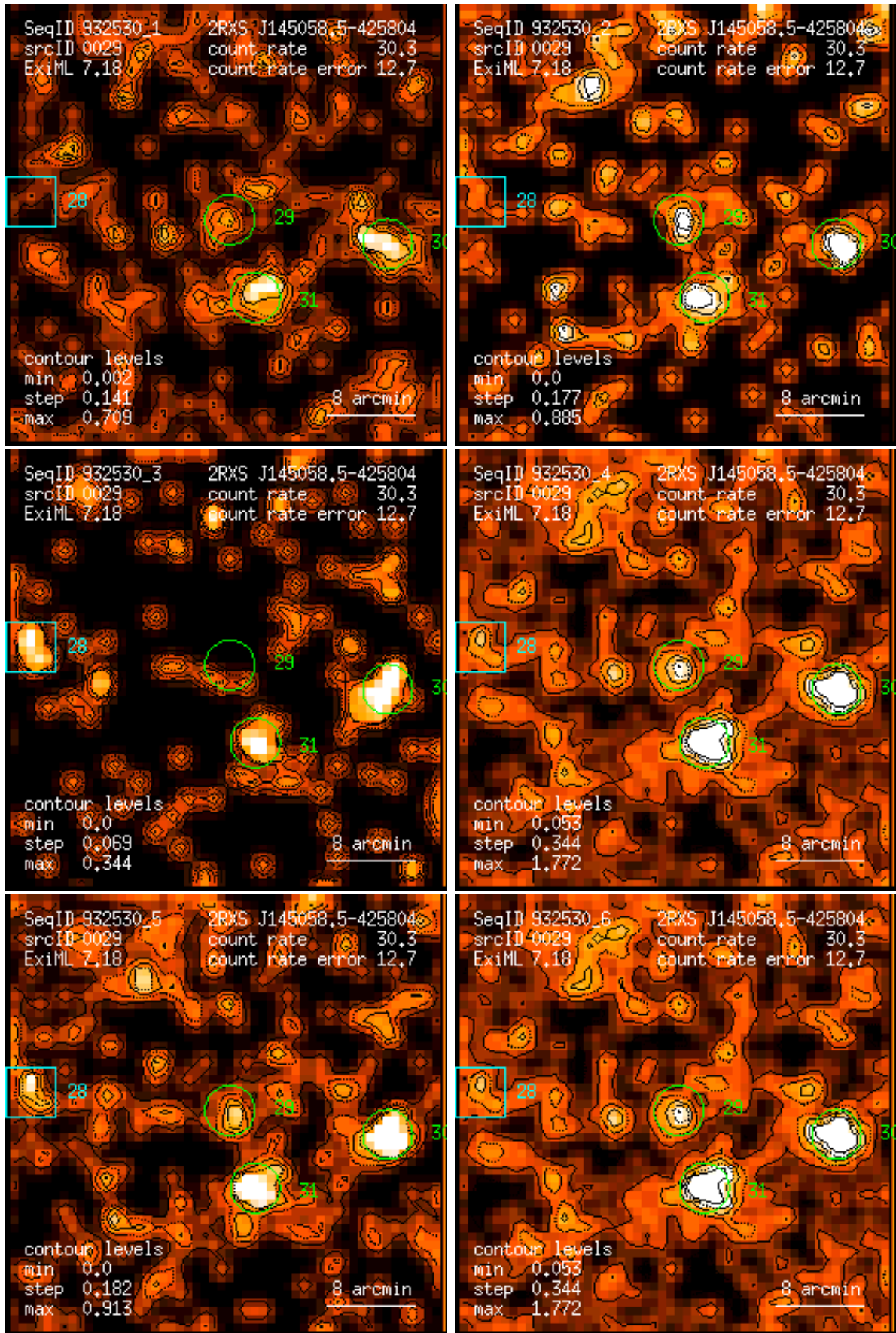
Figure 29: RASS 932530: detection 0029: band rate images, Gaussian filter: (1) PSPC channels 11 – 41, (2) 52 – 90, (3) 91 – 201, (4) 11 – 235, (5) 52 – 201, (6) 11 – 201. Broad band rates in counts/ks. Band rate contour levels in counts/ks/arcmin 2 .
