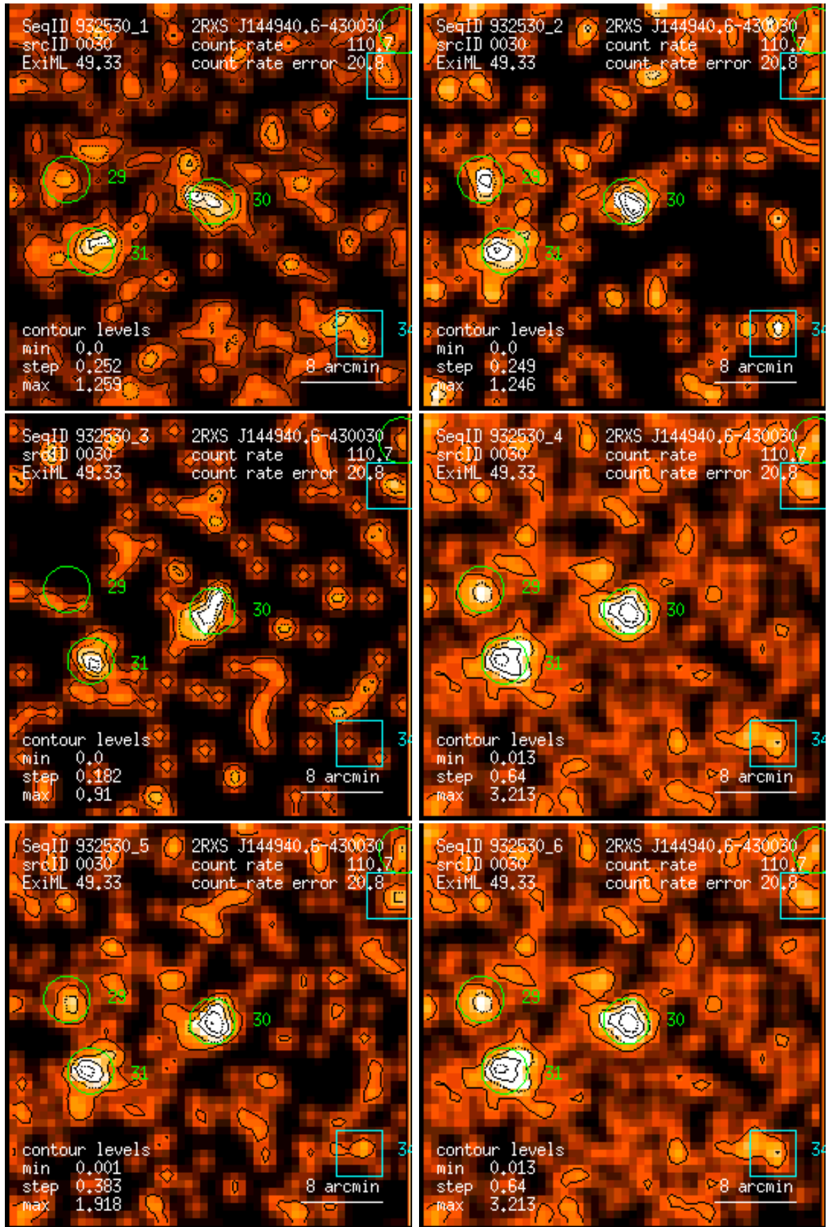
Figure 30: RASS 932530: detection 0030: band rate images, Gaussian filter: (1) PSPC channels 11 – 41, (2) 52 – 90, (3) 91 – 201, (4) 11 – 235, (5) 52 – 201, (6) 11 – 201. Broad band rates in counts/ks. Band rate contour levels in counts/ks/arcmin 2 .
