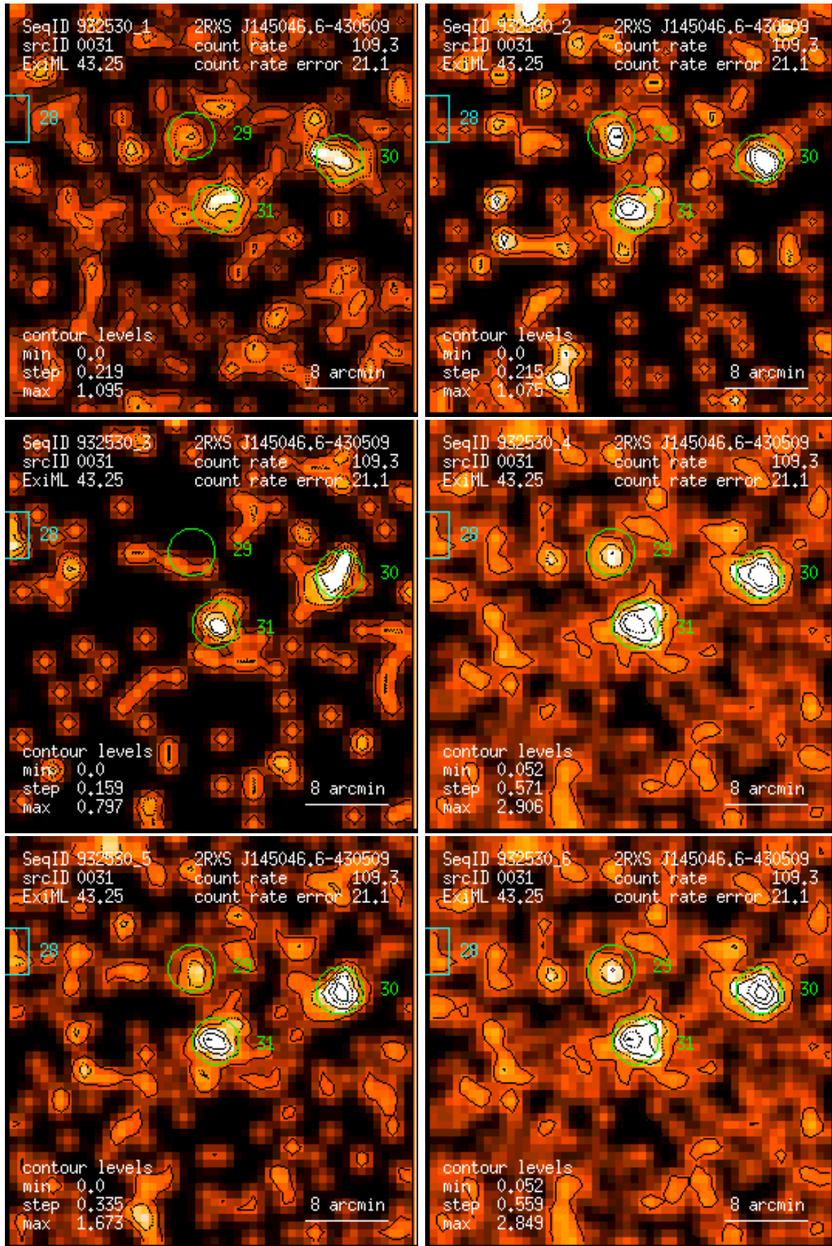
Figure 31: RASS 932530: detection 0031: band rate images, Gaussian filter: (1) PSPC channels 11 – 41, (2) 52 – 90, (3) 91 – 201, (4) 11 – 235, (5) 52 – 201, (6) 11 – 201. Broad band rates in counts/ks. Band rate contour levels in counts/ks/arcmin 2 .
