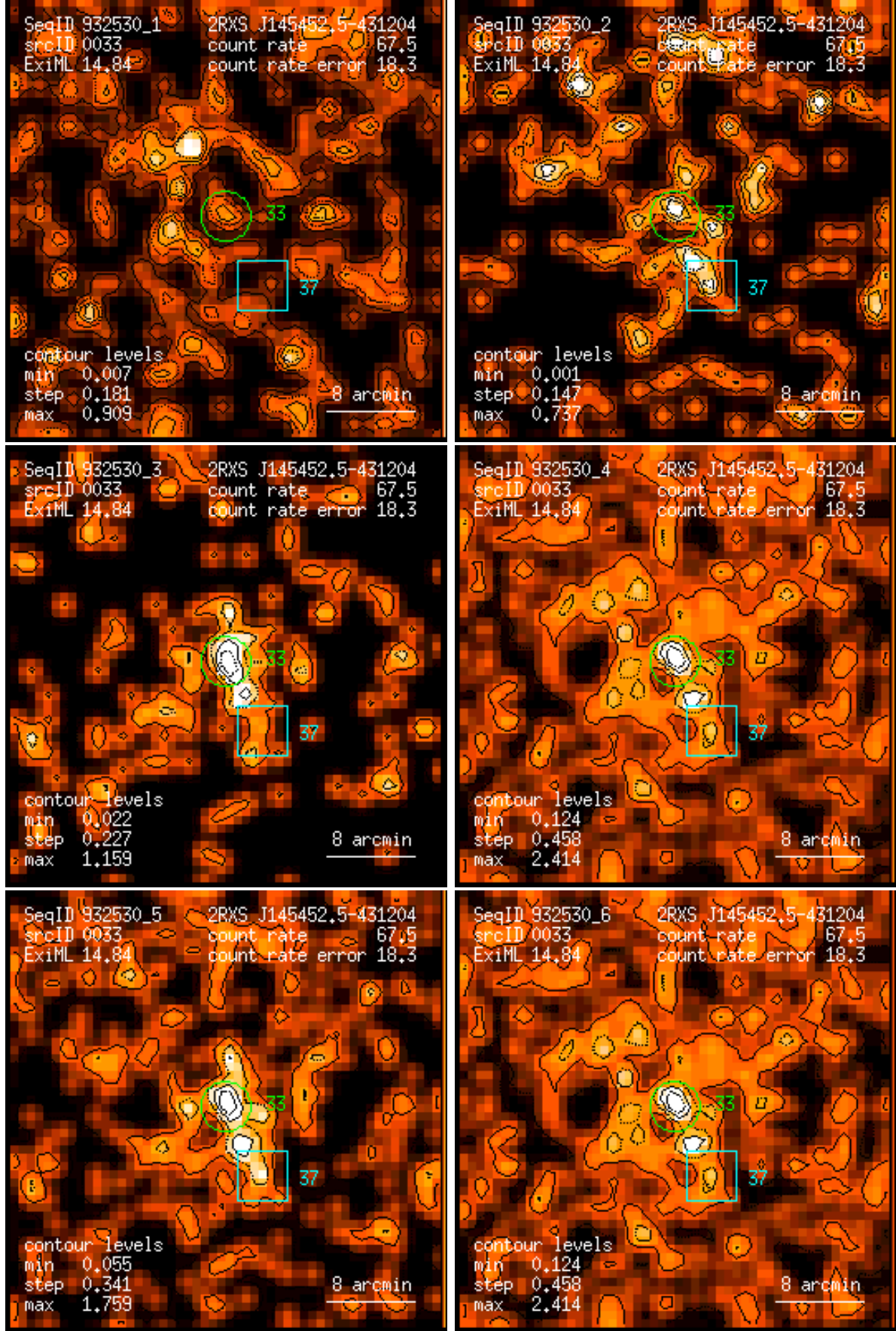
Figure 33: RASS 932530: detection 0033: band rate images, Gaussian filter: (1) PSPC channels 11 – 41, (2) 52 – 90, (3) 91 – 201, (4) 11 – 235, (5) 52 – 201, (6) 11 – 201. Broad band rates in counts/ks. Band rate contour levels in counts/ks/arcmin 2 .
