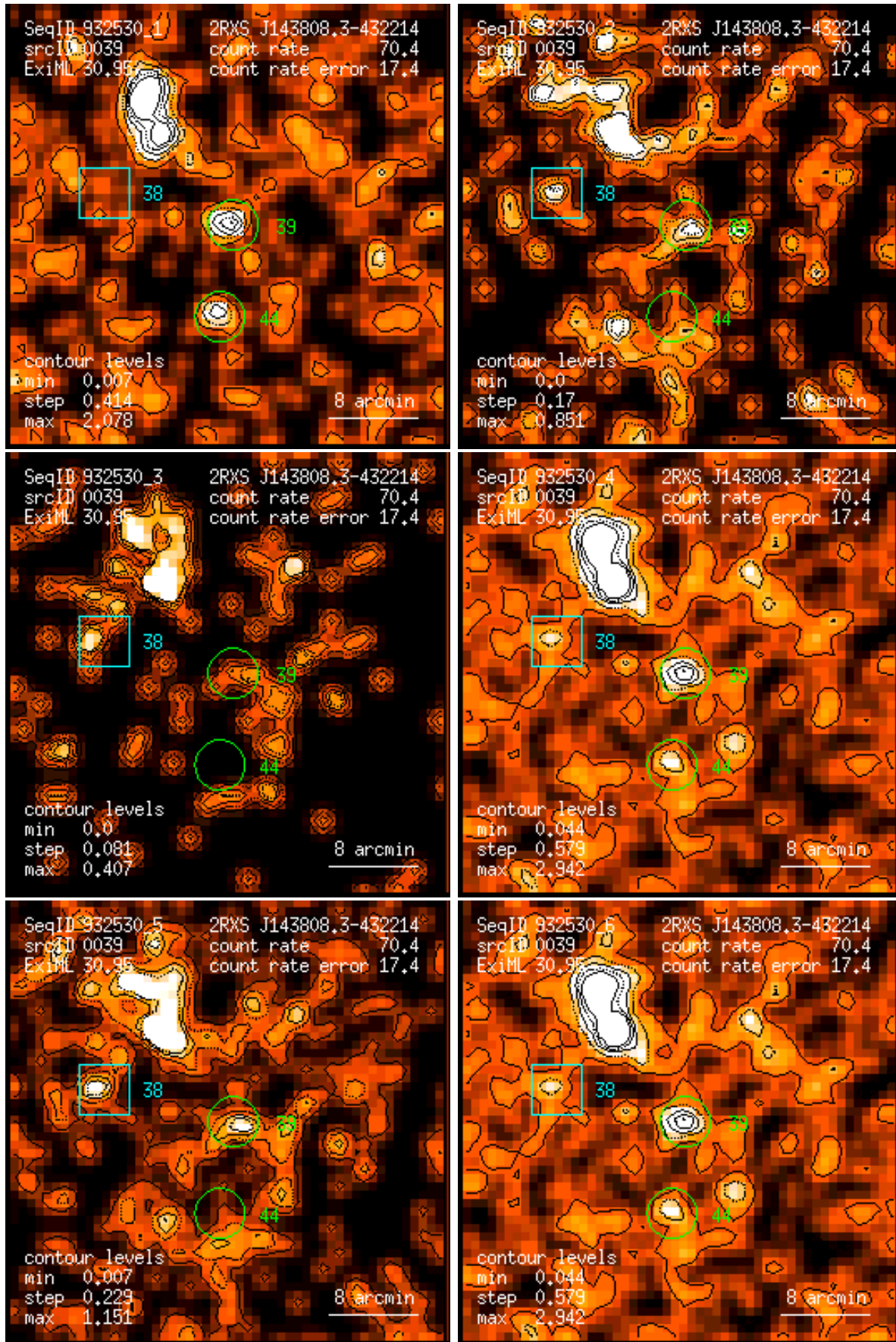
Figure 39: RASS 932530: detection 0039: band rate images, Gaussian filter: (1) PSPC channels 11 – 41, (2) 52 – 90, (3) 91 – 201, (4) 11 – 235, (5) 52 – 201, (6) 11 – 201. Broad band rates in counts/ks. Band rate contour levels in counts/ks/arcmin 2 .
