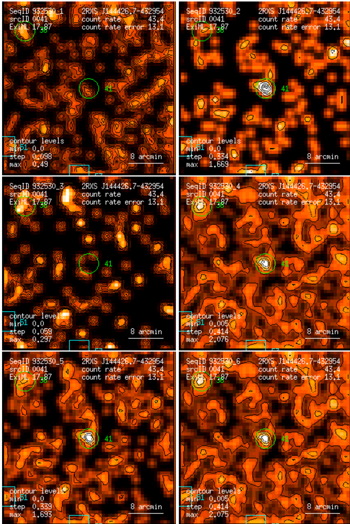
Figure 41: RASS 932530: detection 0041: band rate images, Gaussian filter: (1) PSPC channels 11 – 41, (2) 52 – 90, (3) 91 – 201, (4) 11 – 235, (5) 52 – 201, (6) 11 – 201. Broad band rates in counts/ks. Band rate contour levels in counts/ks/arcmin 2 .
