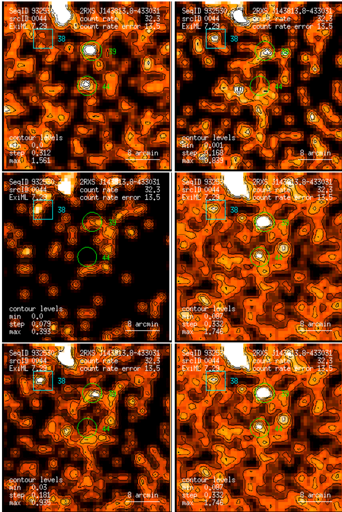
Figure 44: RASS 932530: detection 0044: band rate images, Gaussian filter: (1) PSPC channels 11 – 41, (2) 52 – 90, (3) 91 – 201, (4) 11 – 235, (5) 52 – 201, (6) 11 – 201. Broad band rates in counts/ks. Band rate contour levels in counts/ks/arcmin 2 .
