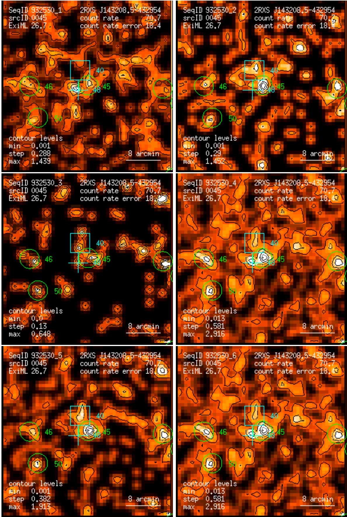
Figure 45: RASS 932530: detection 0045: band rate images, Gaussian filter: (1) PSPC channels 11 – 41, (2) 52 – 90, (3) 91 – 201, (4) 11 – 235, (5) 52 – 201, (6) 11 – 201. Broad band rates in counts/ks. Band rate contour levels in counts/ks/arcmin 2 .
