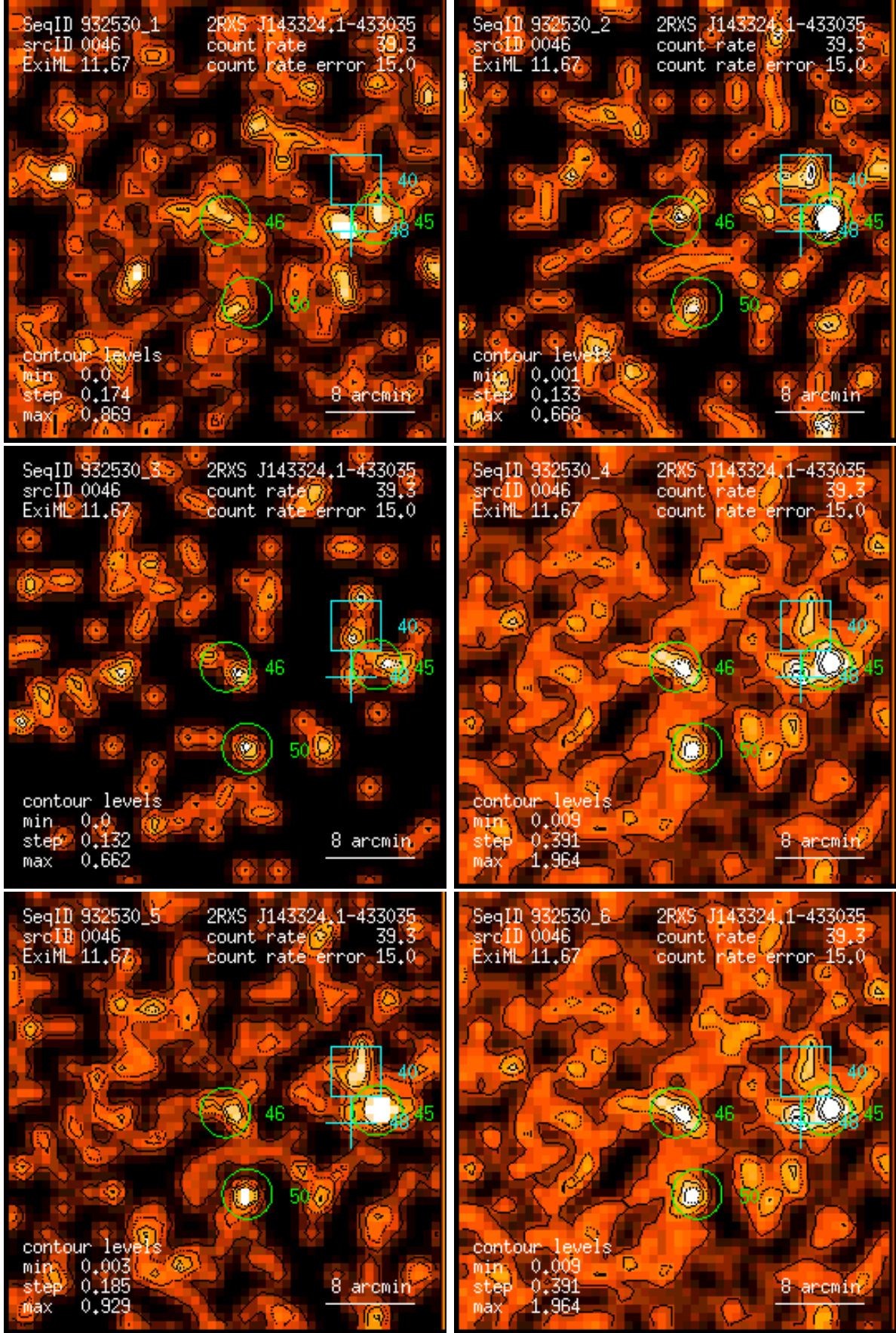
Figure 46: RASS 932530: detection 0046: band rate images, Gaussian filter: (1) PSPC channels 11 – 41, (2) 52 – 90, (3) 91 – 201, (4) 11 – 235, (5) 52 – 201, (6) 11 – 201. Broad band rates in counts/ks. Band rate contour levels in counts/ks/arcmin 2 .
