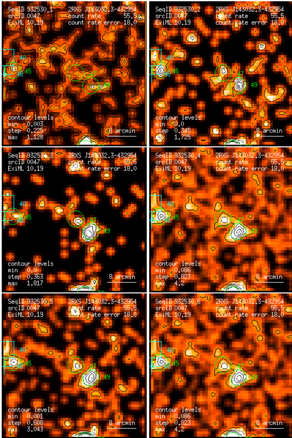
Figure 47: RASS 932530: detection 0047: band rate images, Gaussian filter: (1) PSPC channels 11 – 41, (2) 52 – 90, (3) 91 – 201, (4) 11 – 235, (5) 52 – 201, (6) 11 – 201. Broad band rates in counts/ks. Band rate contour levels in counts/ks/arcmin 2 .
