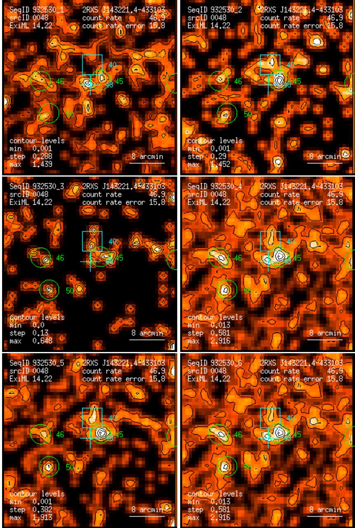
Figure 48: RASS 932530: detection 0048: band rate images, Gaussian filter: (1) PSPC channels 11 – 41, (2) 52 – 90, (3) 91 – 201, (4) 11 – 235, (5) 52 – 201, (6) 11 – 201. Broad band rates in counts/ks. Band rate contour levels in counts/ks/arcmin 2 .
