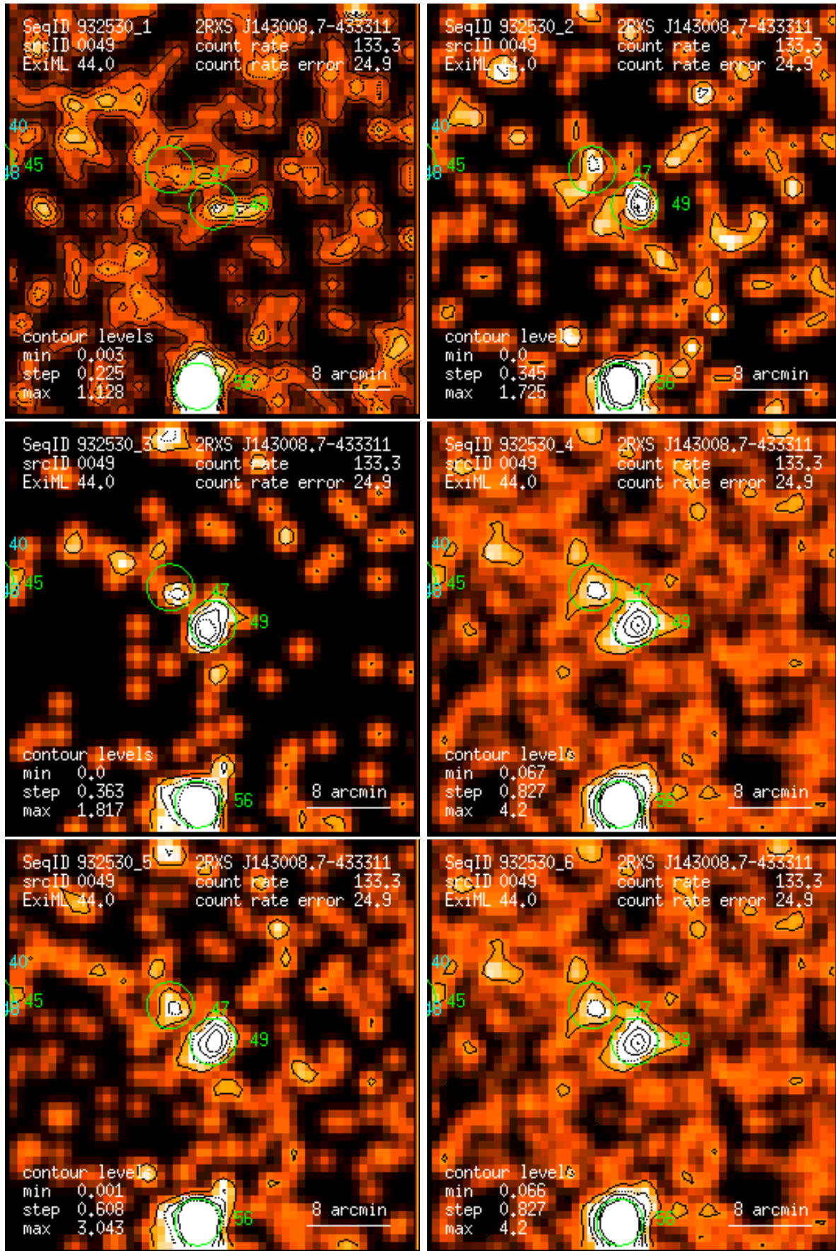
Figure 49: RASS 932530: detection 0049: band rate images, Gaussian filter: (1) PSPC channels 11 – 41, (2) 52 – 90, (3) 91 – 201, (4) 11 – 235, (5) 52 – 201, (6) 11 – 201. Broad band rates in counts/ks. Band rate contour levels in counts/ks/arcmin 2 .
