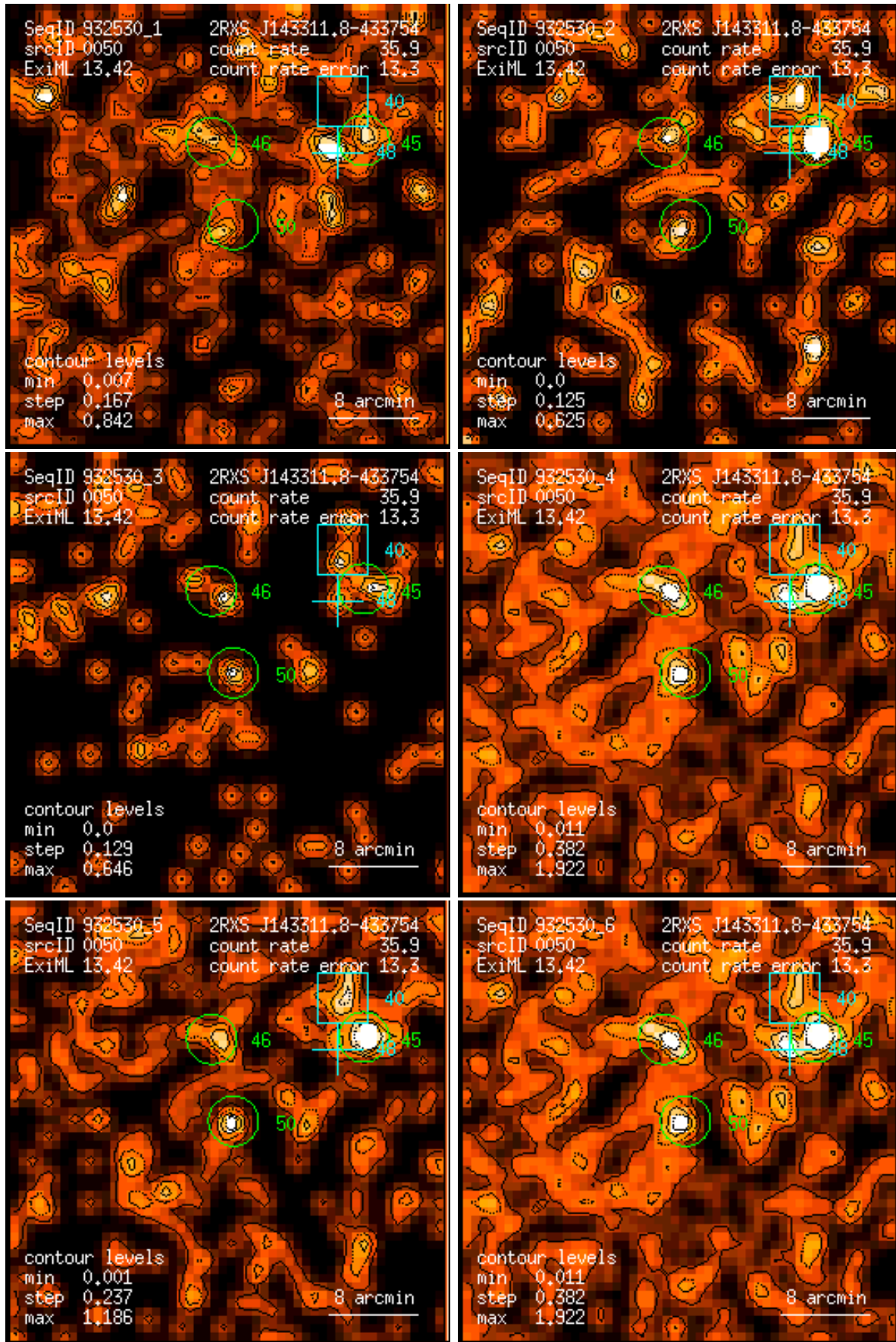
Figure 50: RASS 932530: detection 0050: band rate images, Gaussian filter: (1) PSPC channels 11 – 41, (2) 52 – 90, (3) 91 – 201, (4) 11 – 235, (5) 52 – 201, (6) 11 – 201. Broad band rates in counts/ks. Band rate contour levels in counts/ks/arcmin 2 .
