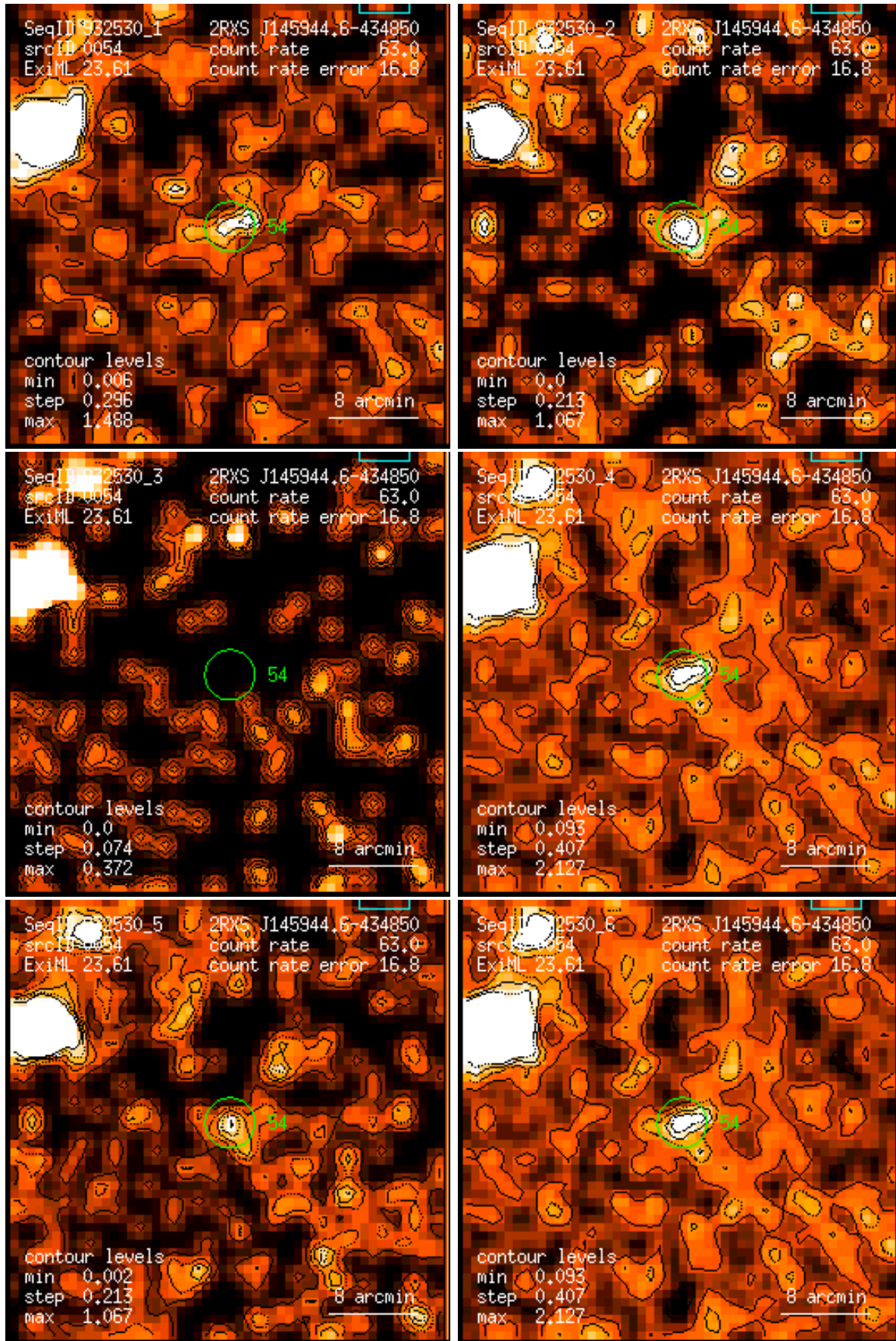
Figure 54: RASS 932530: detection 0054: band rate images, Gaussian filter: (1) PSPC channels 11 – 41, (2) 52 – 90, (3) 91 – 201, (4) 11 – 235, (5) 52 – 201, (6) 11 – 201. Broad band rates in counts/ks. Band rate contour levels in counts/ks/arcmin 2 .
